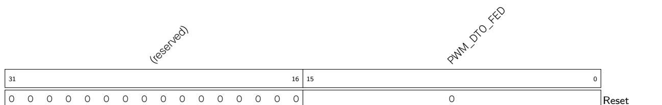
Register 16.24. PWM_DTO_FED_CFG_REG (0x005c)
