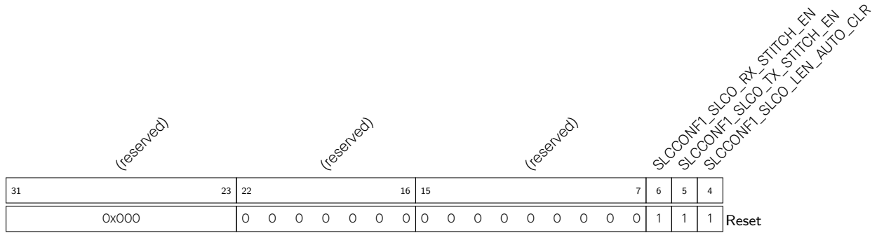
Register 8.10. SLCCONF1_REG (0x60)
