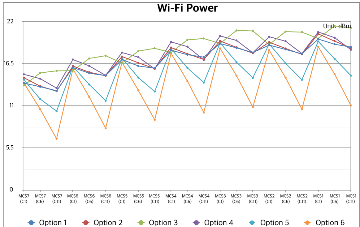
Figure 2. Wi-Fi Power Values for Six Placement Options
