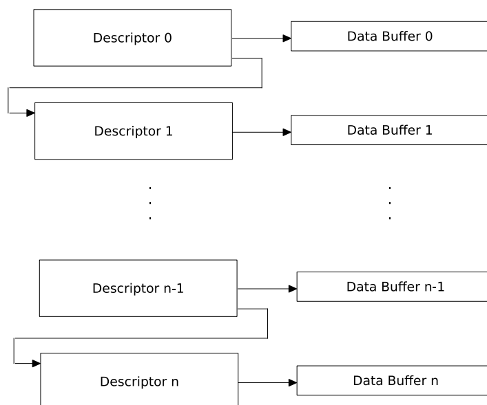
Figure 34.5-6. DMA Linked List of the SDIO Slave
