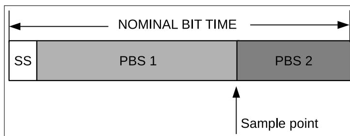
Figure 33.2-5. Layout of a Bit
