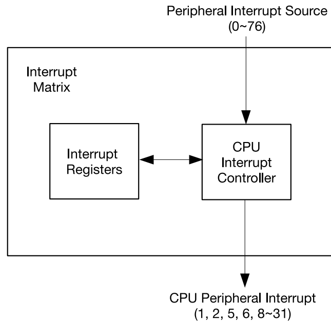
Figure 10.2-1. Interrupt Matrix Structure
