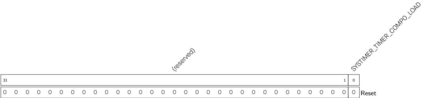
Register 13.17. SYSTIMER_COMPO_LOAD_REG (0x0050)
