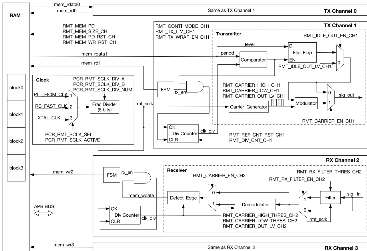
Figure 37.3-1. RMT Architecture
