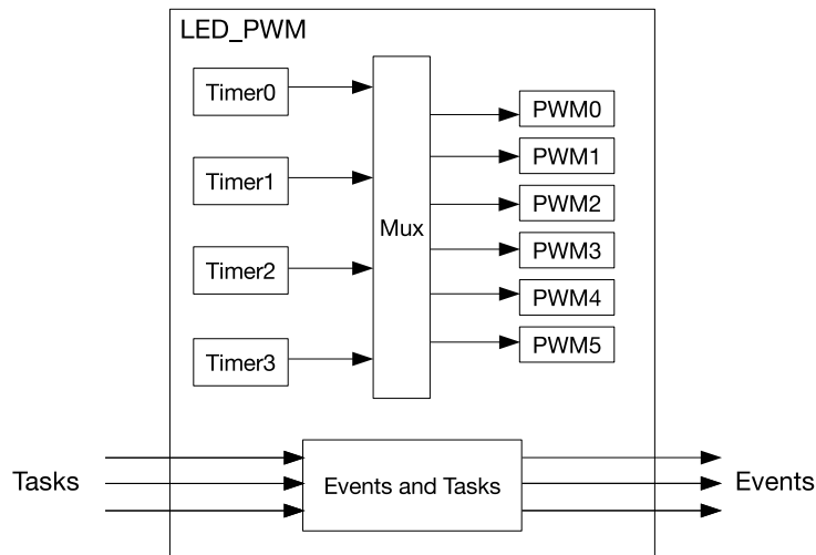
Figure 35.2-1. LED PWM Architecture
