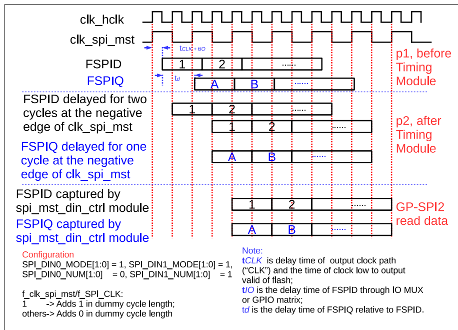
Figure 28.8-2. Timing Compensation Example in GP-SPI2 as Master
