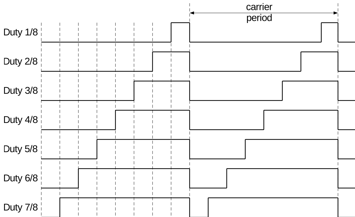
Figure 36.3-30. Possible Duty Cycle Settings for Sustaining Pulses in the PWM Carrier Submodule
