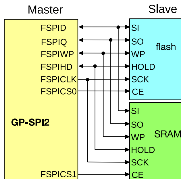
Figure 28.5-7. Connection of GP-SPI2 to Flash and External RAM in 4-bit Mode
