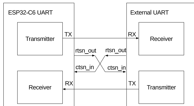
Figure 27.4-9. Connection between Hardware Flow Control Signals
