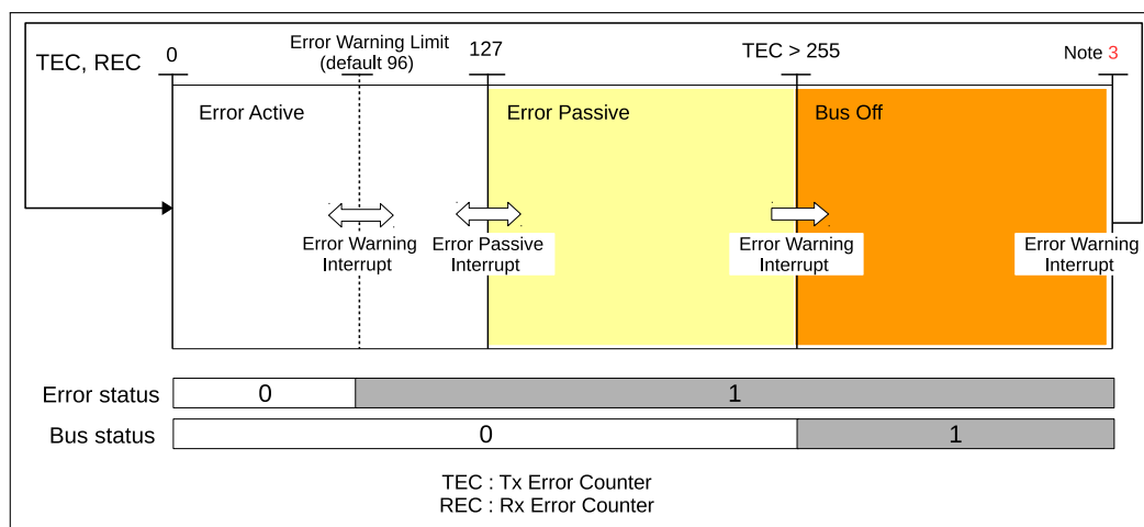
Figure 33.4-4. Error State Transition
