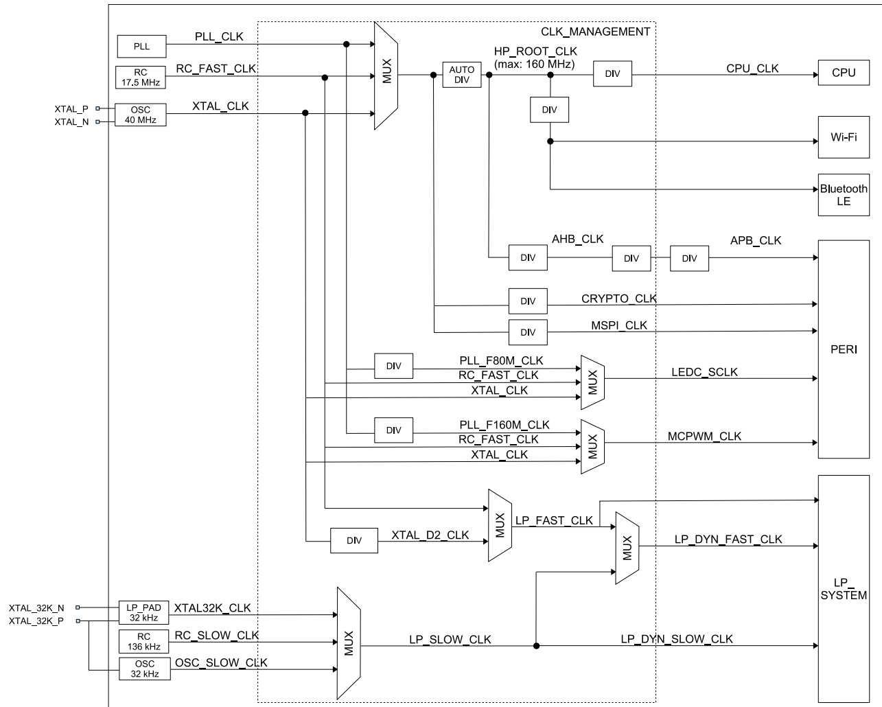
Figure 8.2-1. System Clock
