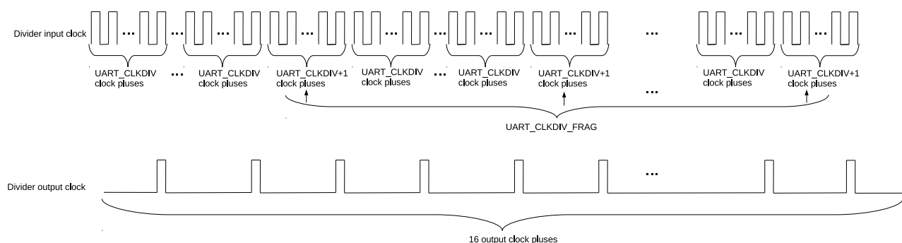
Figure 27.4-1. UART Controllers Division
