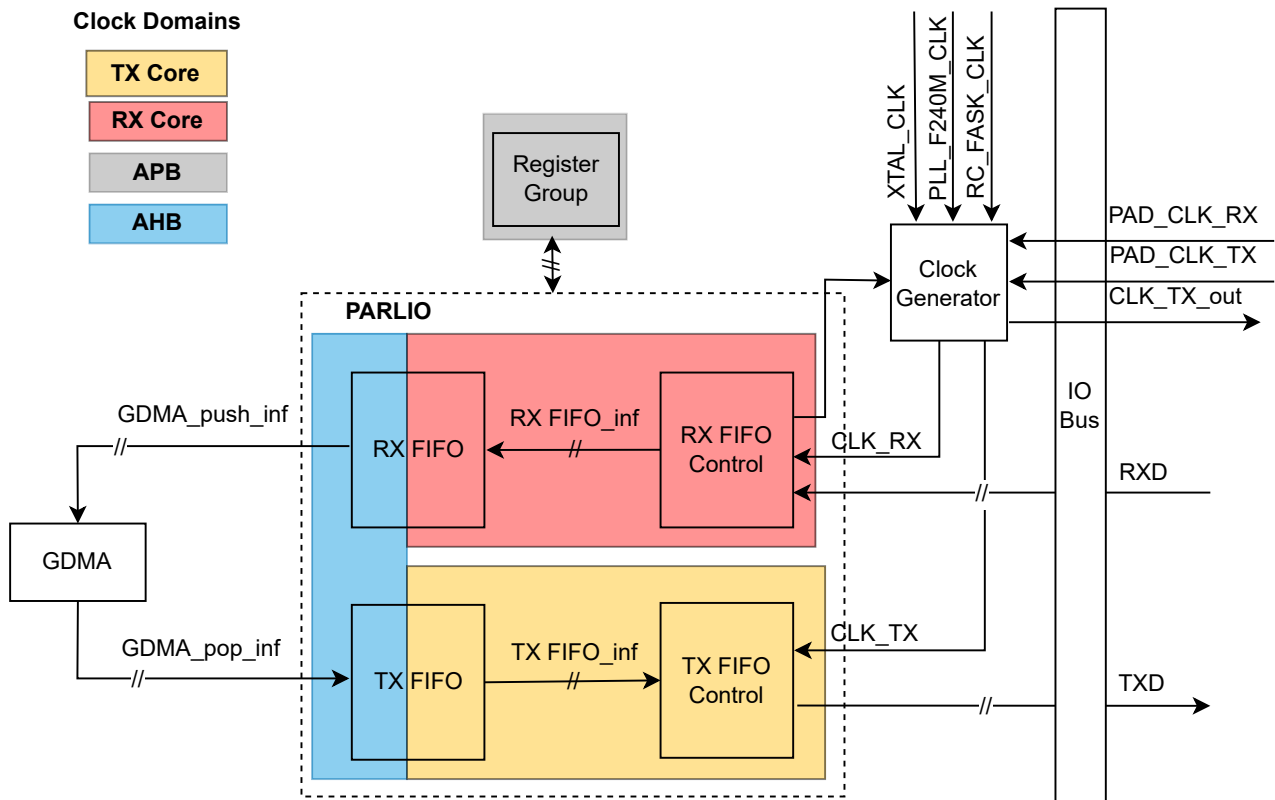
Figure 38.4-1. PARLIO Architecture
