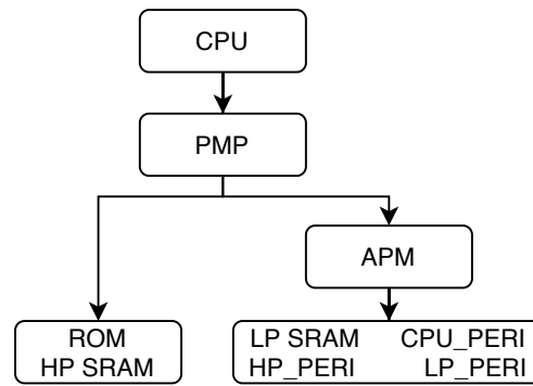
Figure 16.1-1. PMP-APM Management Relation
