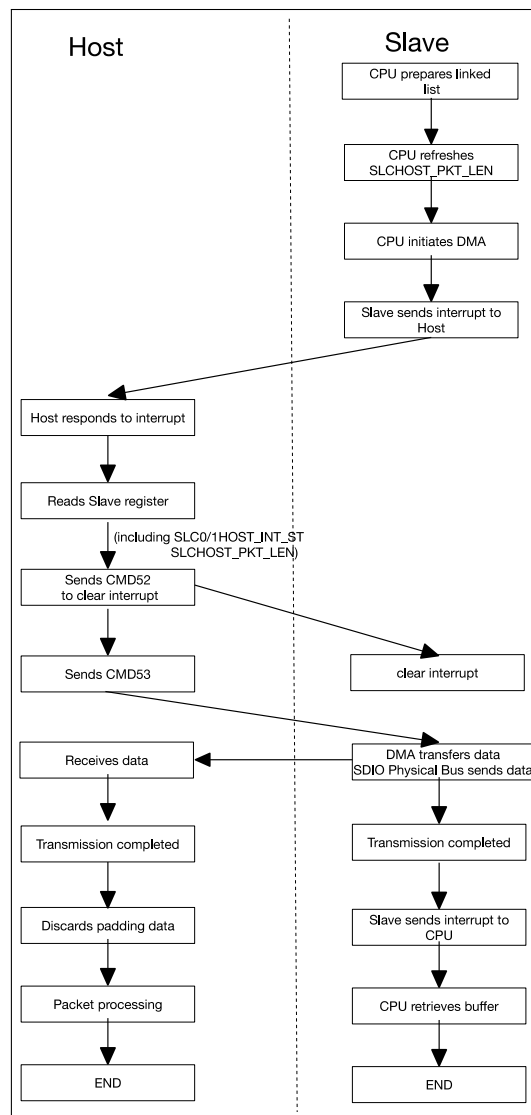
Figure 34.7-1. Procedure of Slave Sending Packets to Host
