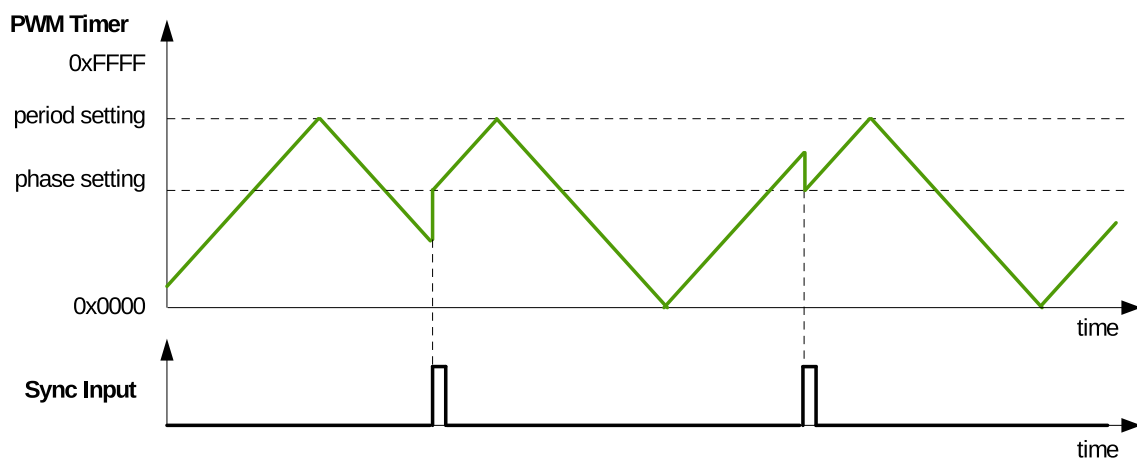
Figure 36.3-10. Count-Up-Down Mode Waveforms, Count-Up at Synchronization Event
