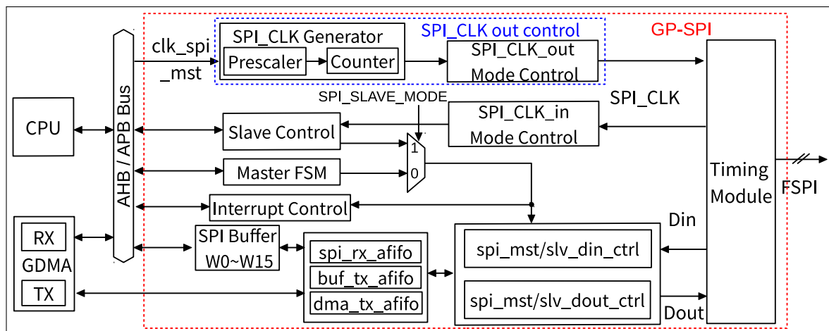
Figure 28.5-2. GP-SPI2 Block Diagram
