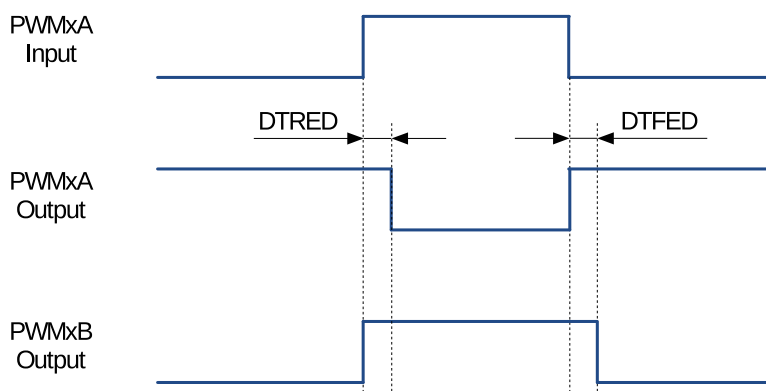
Figure 36.3-25. Active Low Complementary (ALC) Dead Time Waveforms
