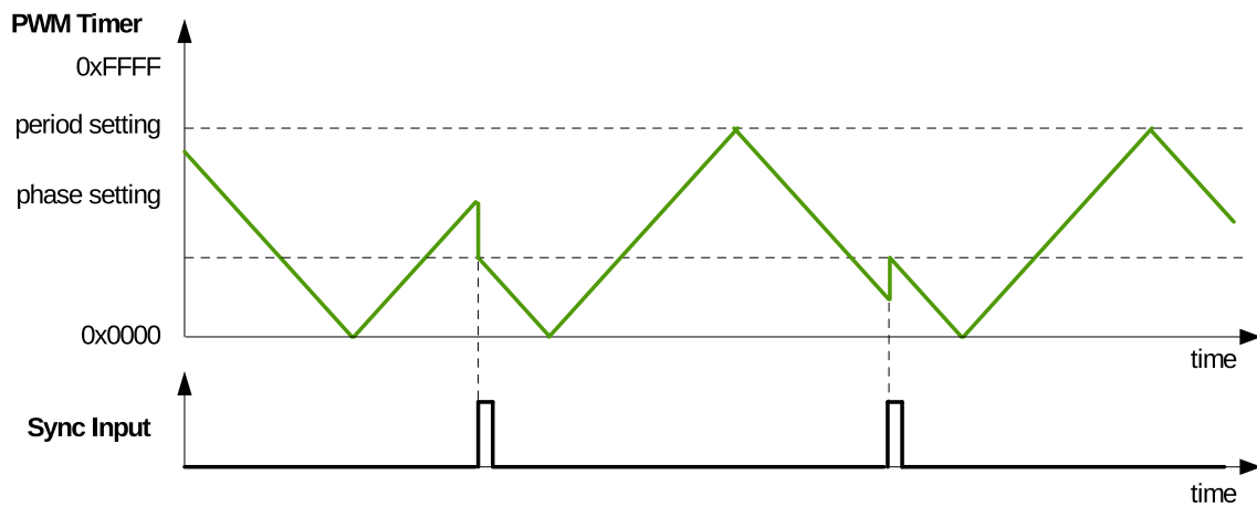
Figure 36.3-9. Count-Up-Down Mode Waveforms, Count-Down at Synchronization Event
