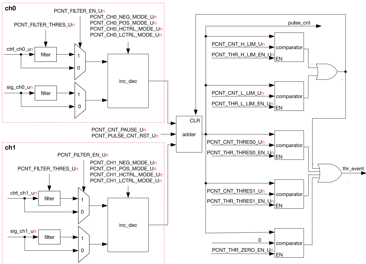
Figure 31.2-1. PCNT Unit Architecture
