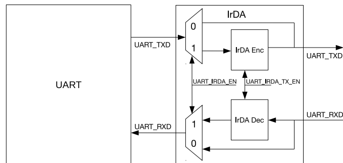
Figure 27.4-7. IrDA Encoding and Decoding Diagram
