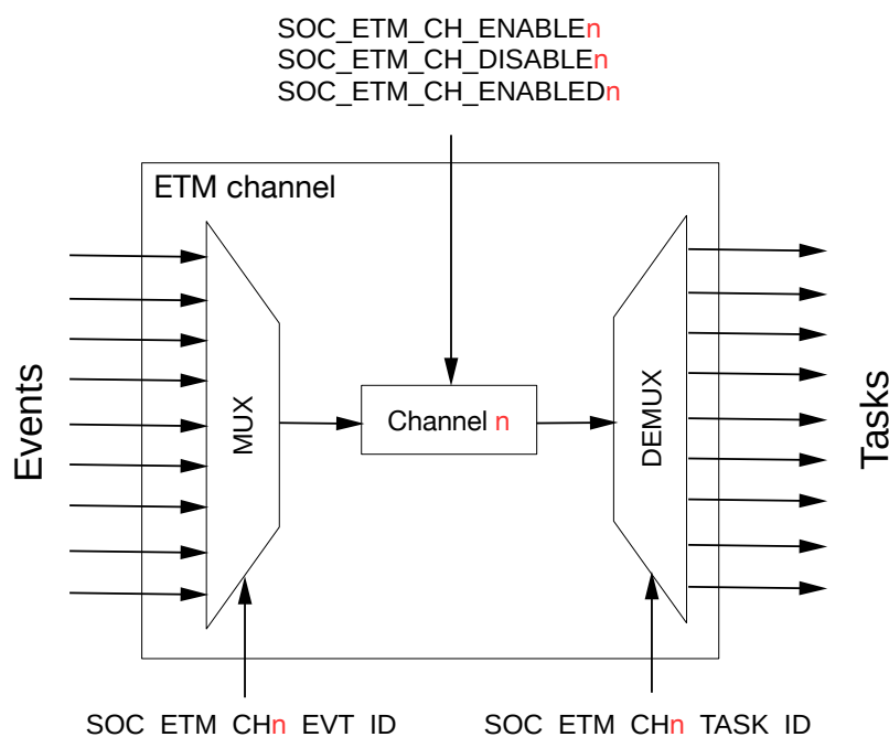
Figure 11.3-2. ETM Channel n Architecture
