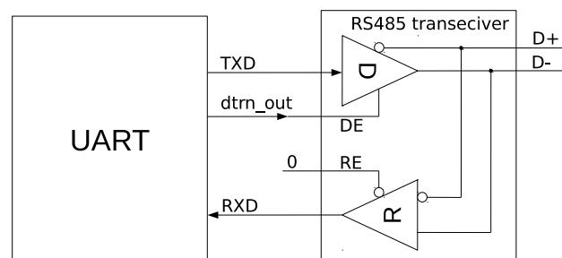
Figure 27.4-5. Driver Control Diagram in RS485 Mode
