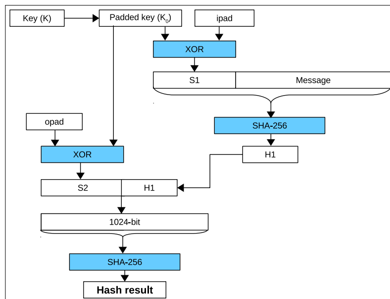
Figure 21.3-2. HMAC Structure Schematic Diagram
