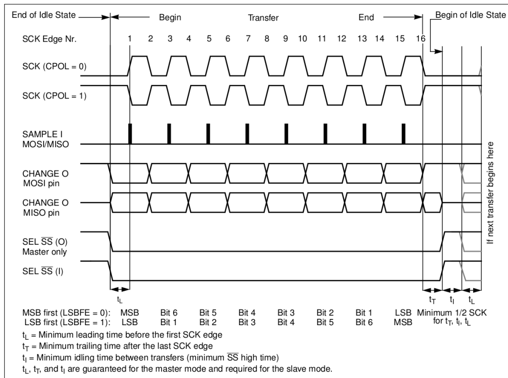
Figure 28.7-1. SPI Clock Mode 0 or 2
