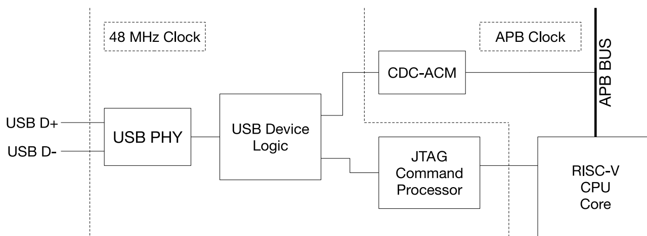
Figure 32.2-1. USB Serial/JTAG High Level Diagram
