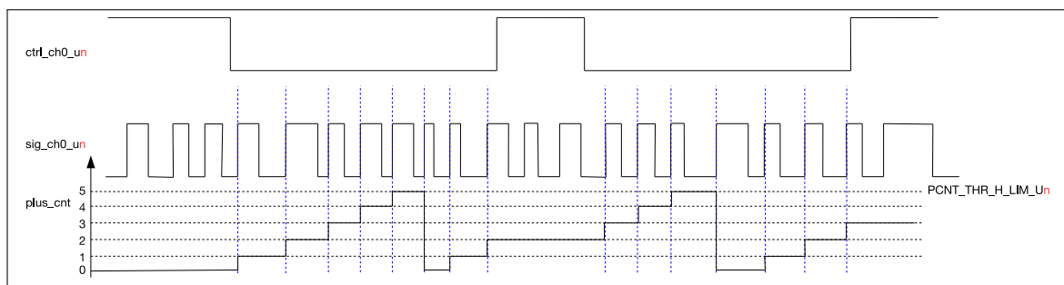
Figure 31.3-1. Channel 0 Up Counting Diagram
