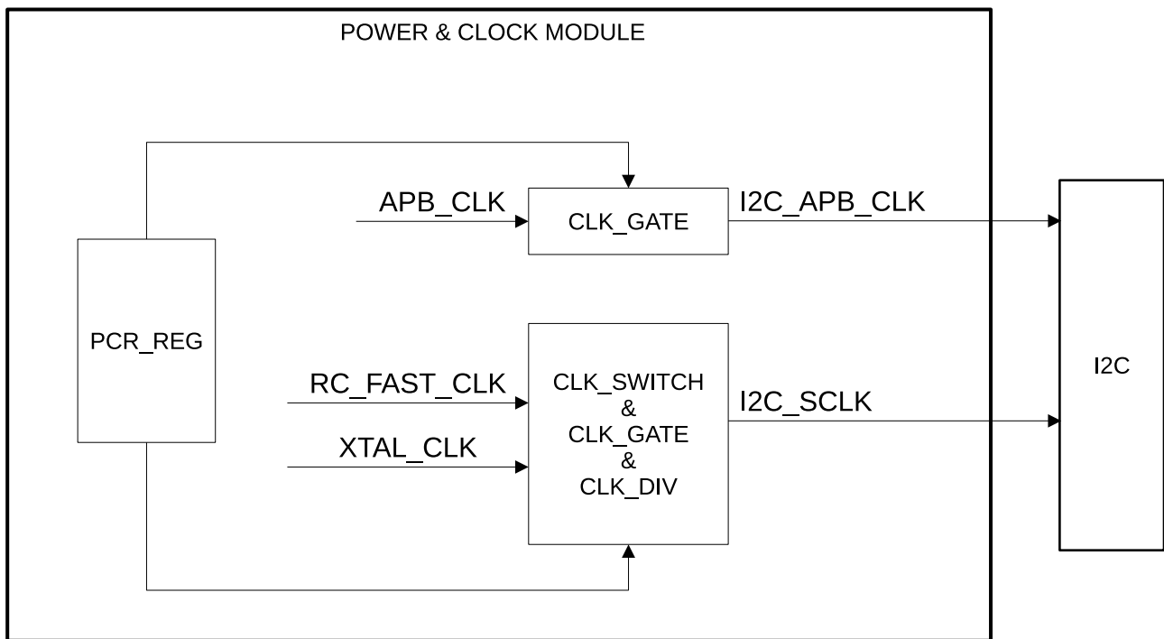
Figure 8.3-1. Clock Configuration Example
