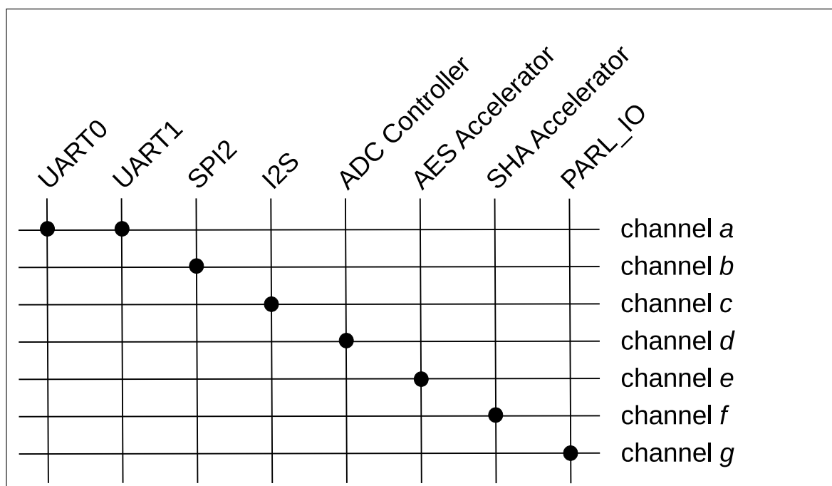
Figure 5.3-2. Modules/peripherals that can work with GDMA
