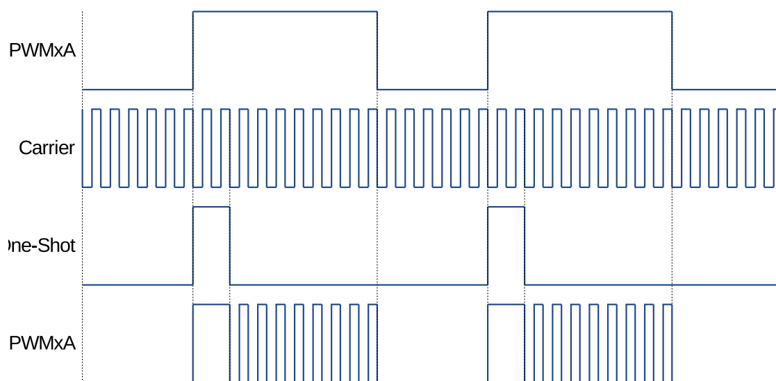
Figure 36.3-29. Example of the First Pulse and the Subsequent Sustaining Pulses of the PWM Carrier Submodule
