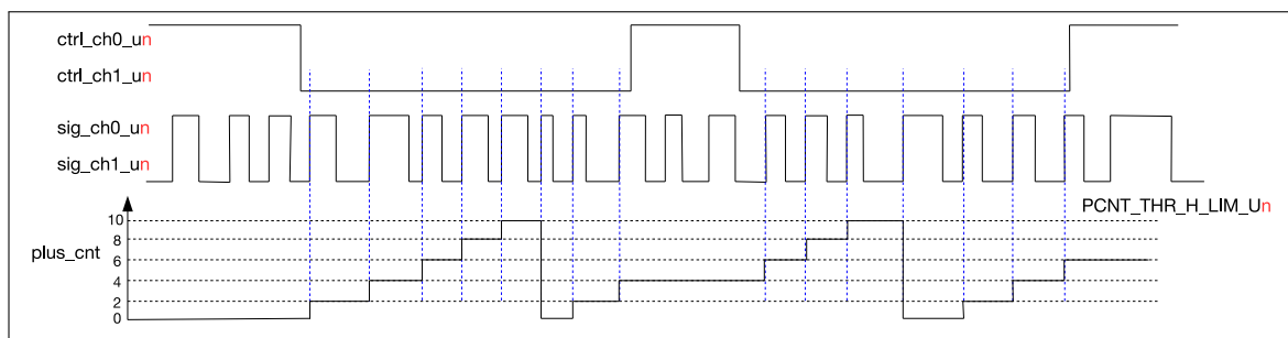
Figure 31.3-3. Two Channels Up Counting Diagram
