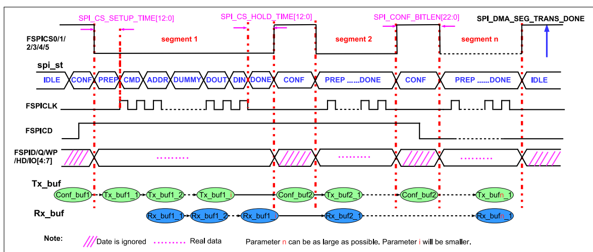
Figure 28.5-9. Configurable Segmented Transfer as Master
