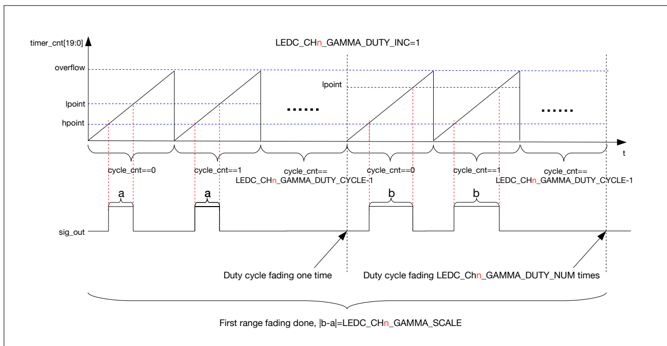
Figure 35.3-5. Output Signal of Linear Duty Cycle Fading
