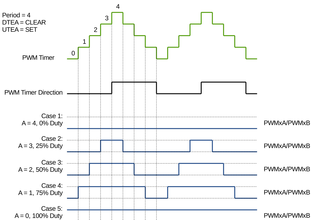
Figure 36.3-15. Symmetrical Waveform in Count-Up-Down Mode
