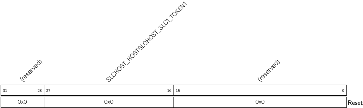
Register 34.52. SLCHOST_SLC1HOST_TOKEN_RDATA_REG (0x00C4)
