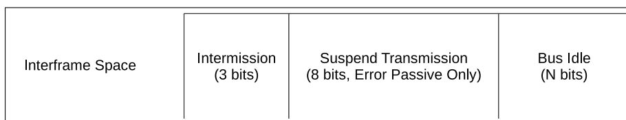
Figure 33.2-4. The Fields within an Interframe Space
