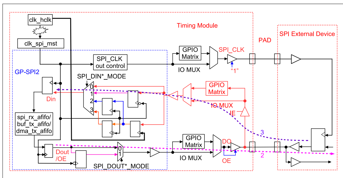
Figure 28.8-1. Timing Compensation Control Diagram in GP-SPI2 as Master
