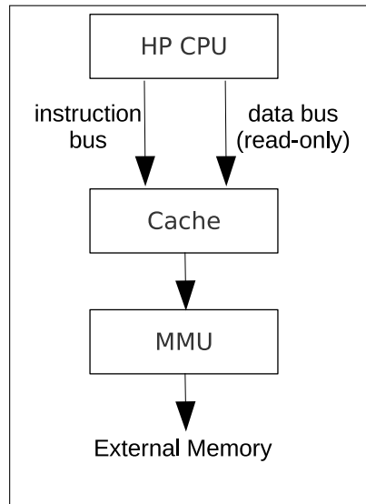
Figure 5.3-1. Cache Structure
