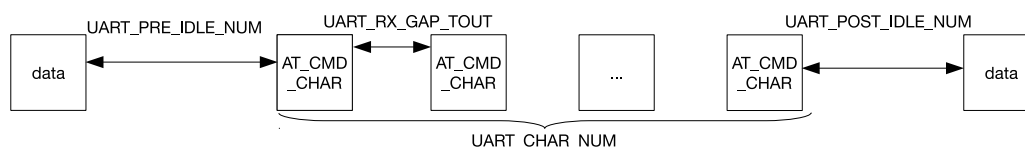
Figure 27.4-4. AT_CMD Character Structure
