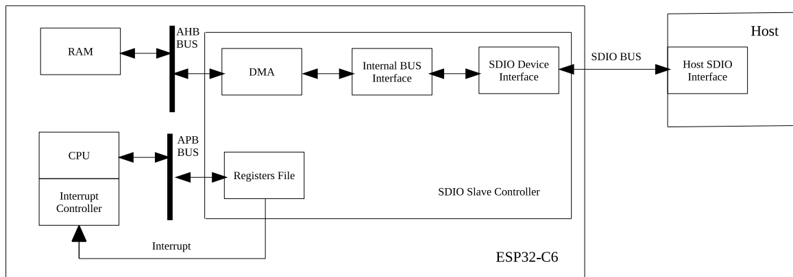
Figure 34.3-1. SDIO Slave Block Diagram
