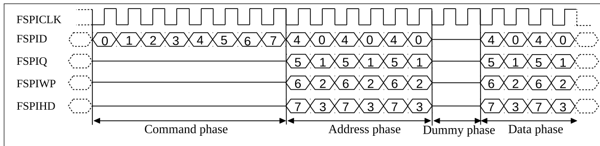
Figure 28.5-8. SPI Quad I/O Read Command Sequence Sent by GP-SPI2 to Flash
