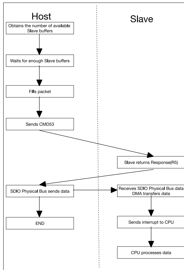
Figure 34.7-2. Procedure of Slave Receiving Packets from Host
