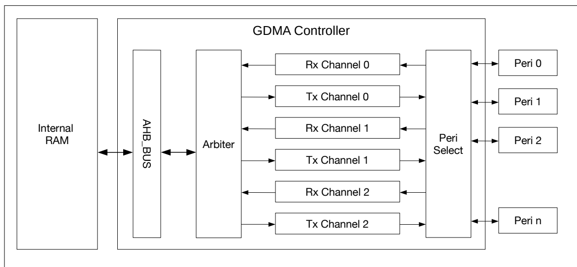
Figure 4.3-1. GDMA controller Architecture
