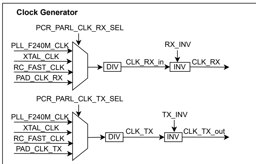
Figure 38.5-1. PARLIO Clock Generation
