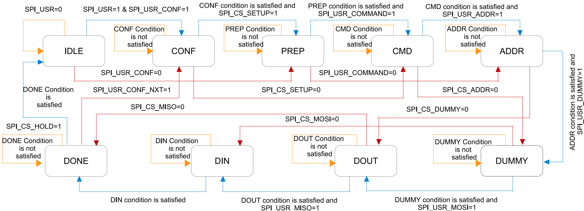
Figure 28.5-5. GP-SPI2 State Machine as Master
