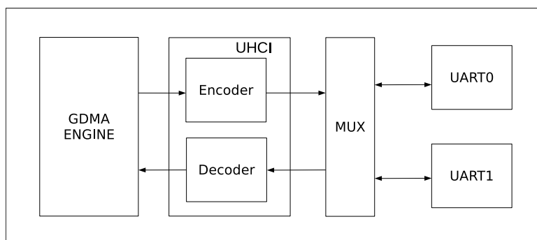
Figure 27.4-10. Data Transfer in GDMA Mode
