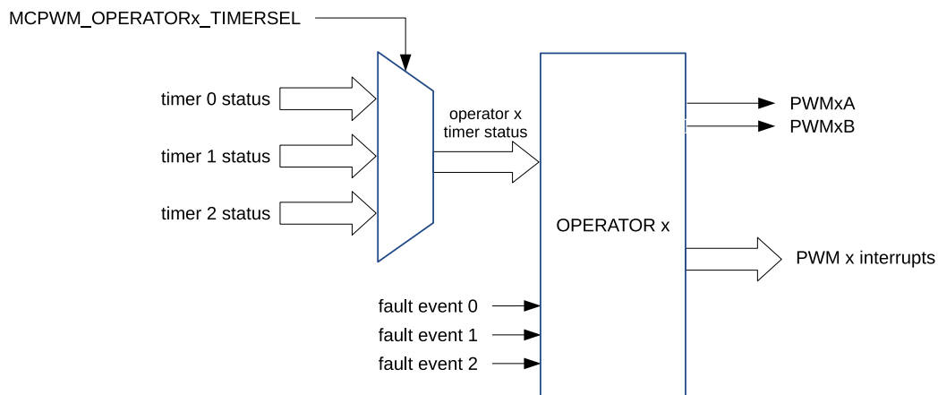
Figure 36.3-3. Operator Module
