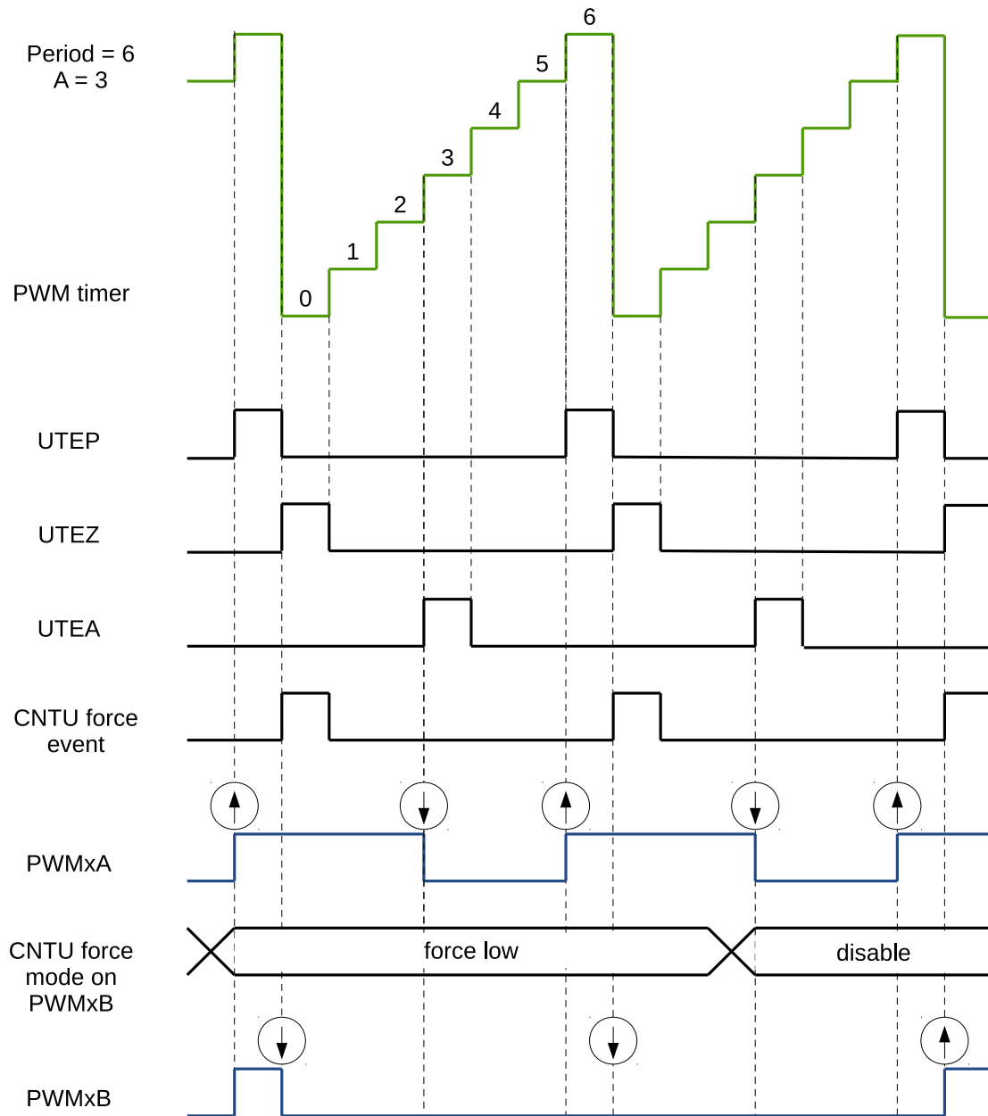
Figure 36.3-22. Example of a CNTU Software-Force Event on PWMxB
