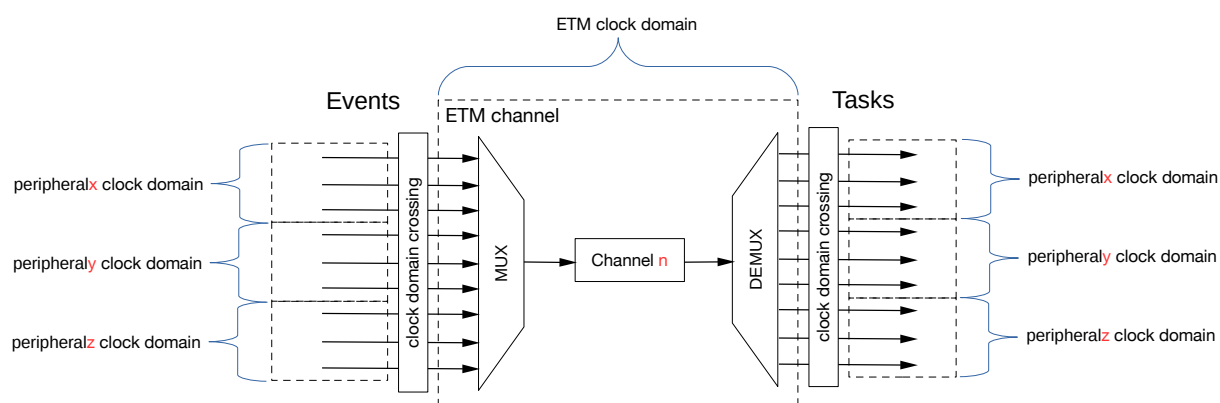
Figure 11.3-3. Event Task Matrix Clock Architecture
