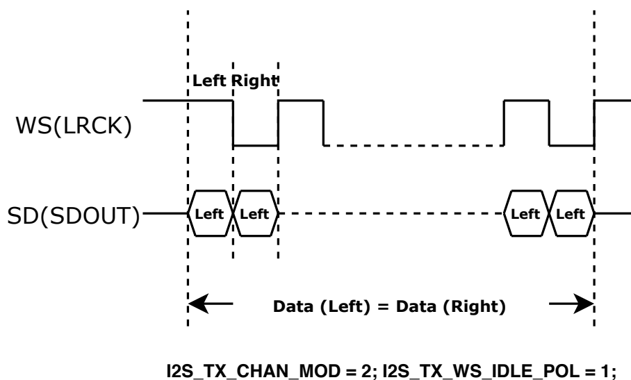
Figure 30.9-3. PDM Channel Control Example
