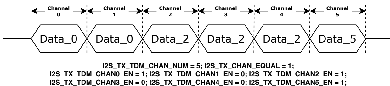
Figure 30.9-2. TDM Channel Control
