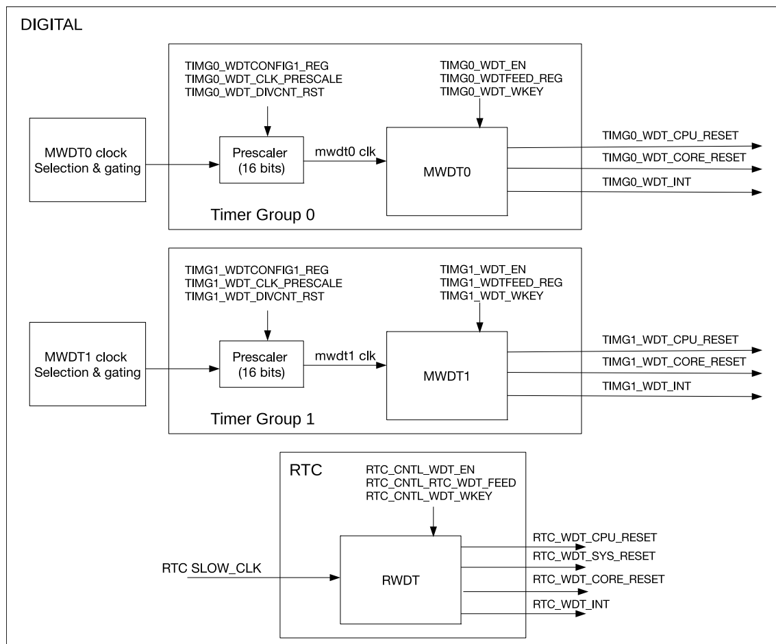
Figure 15.2-1. Digital Watchdog Timers in ESP32-C6
