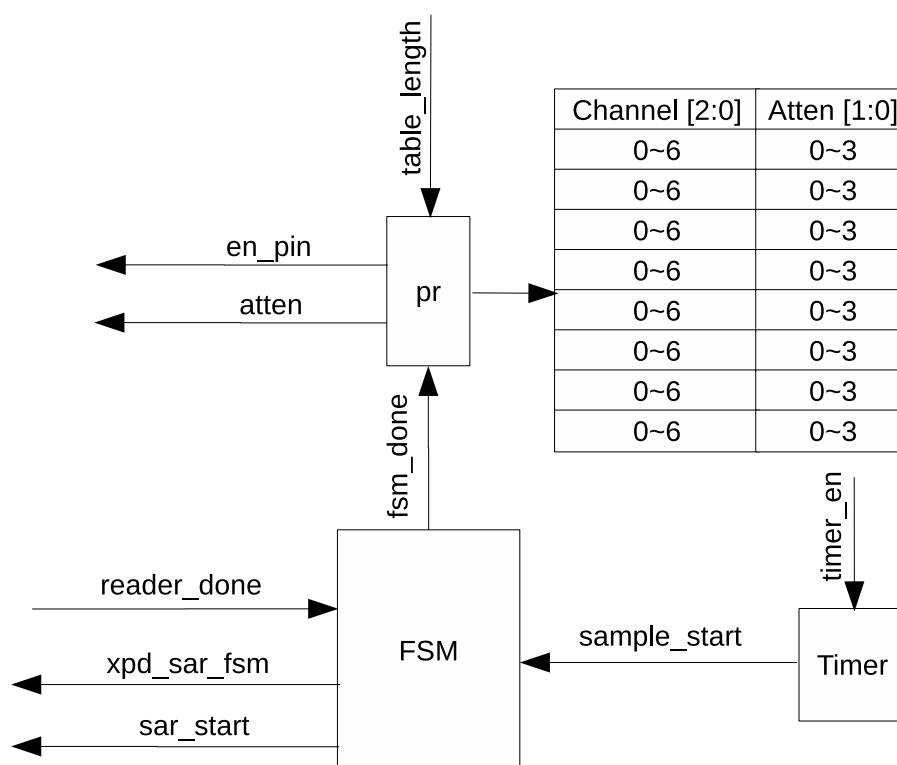
Figure 39.2-2. Diagram of DIG ADC FSM
