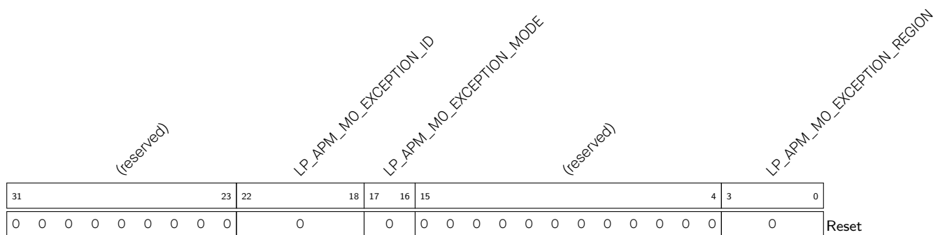
Register 16.32. LP_APM_MO_EXCEPTION_INFO_REG (0x00D0)
