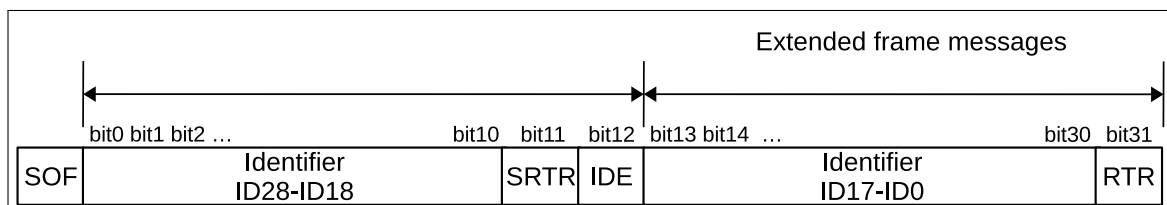
Figure 33.4-5. Positions of Arbitration Lost Bits
