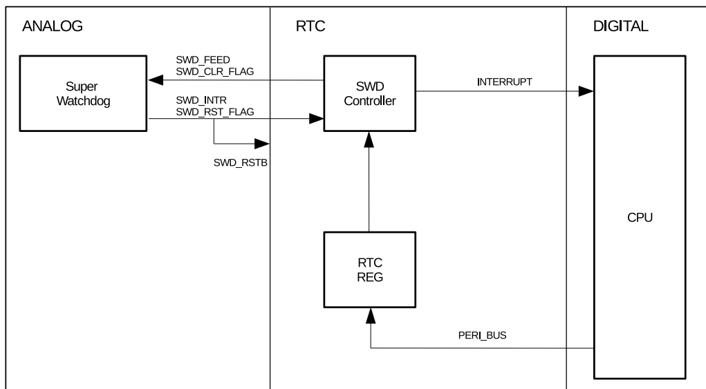
Figure 15.3-1. Super Watchdog Controller Structure
