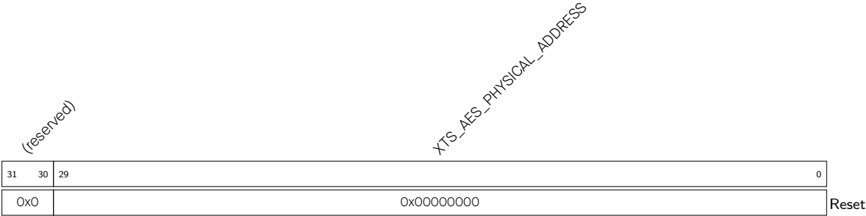
Register 25.4. XTS_AES_PHYSICAL_ADDRESS_REG (0x0348)
