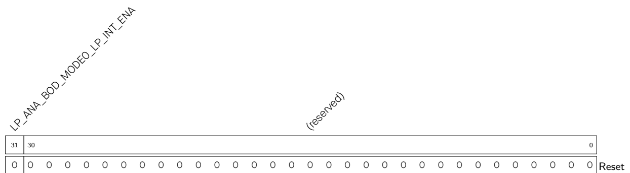
Register 12.89. LP_ANA_LP_INT_ENA_REG (0x0028)
