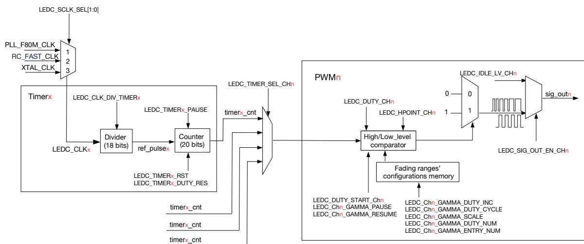
Figure 35.3-1. Timer and PWM Generator Block Diagram
