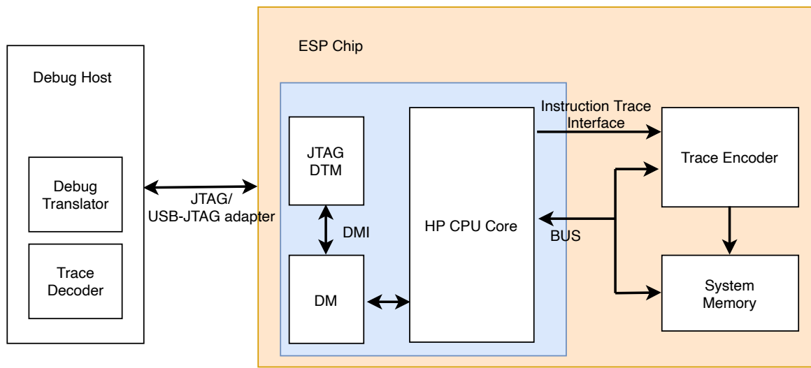
Figure 2.2-1. Trace Overview
