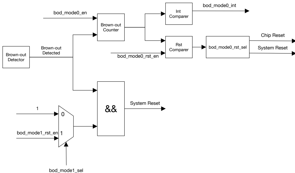
Figure 12.4-3. Brownout Reset Workflow
