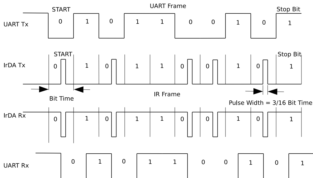
Figure 27.4-6. The Timing Diagram of Encoding and Decoding in SIR mode
