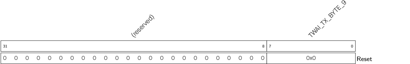
Register 33.14. TWAI_DATA_9_REG (0x0064)
