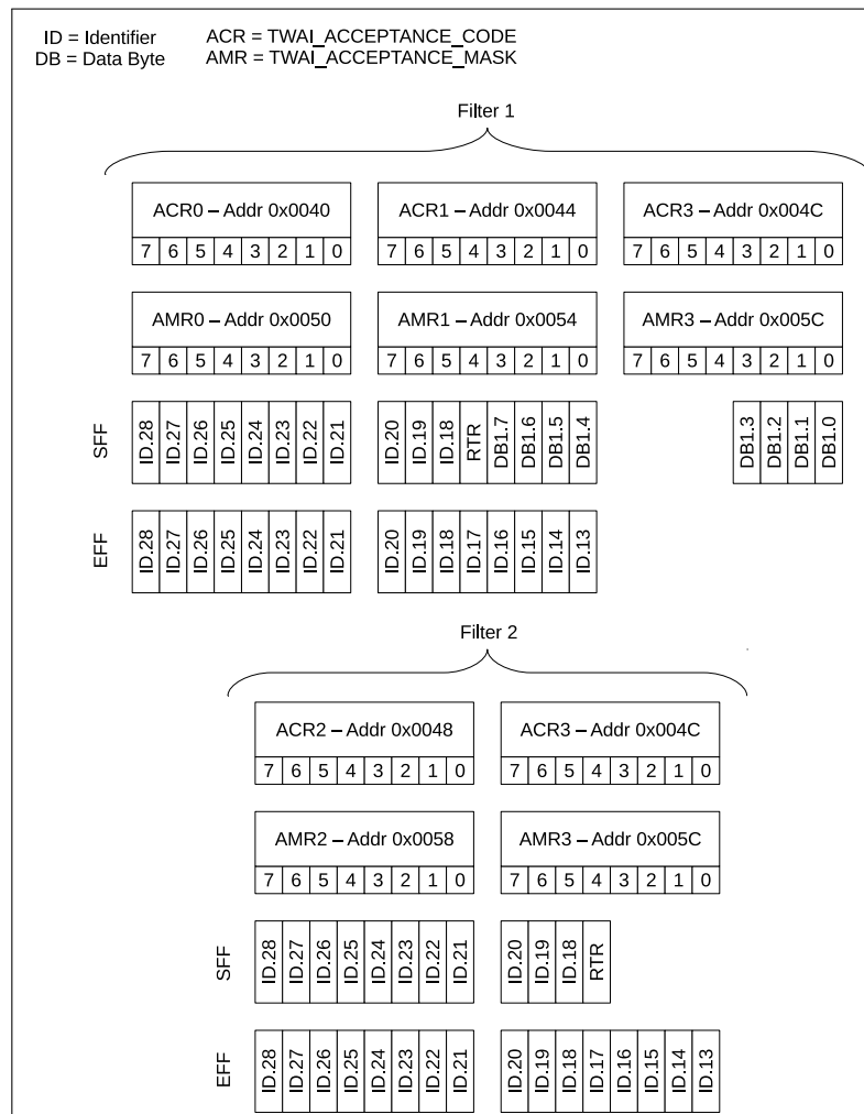
Figure 33.4-3. Dual Filter Mode
