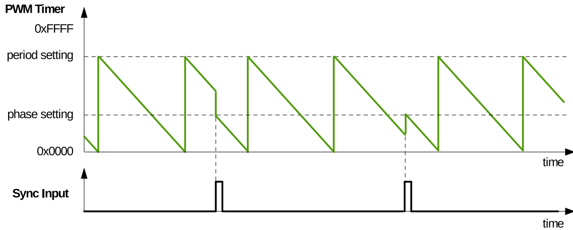
Figure 36.3-8. Count-Down Mode Waveforms
