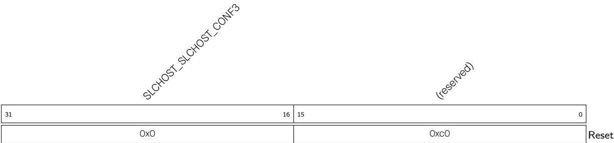
Register 34.54. SLCHOST_CONF_W3_REG (0x0078)
