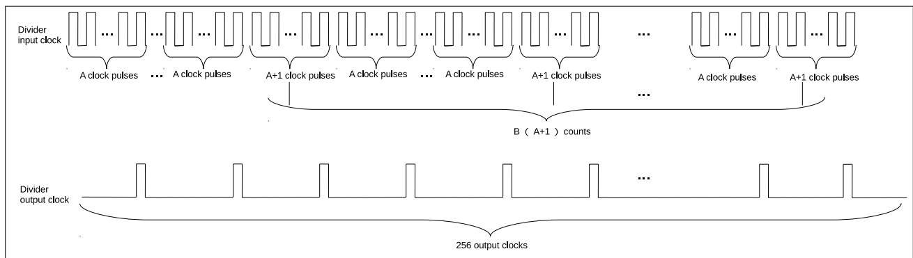
Figure 35.3-2. Frequency Division When LEDC_CLK_DIV is a Non-Integer Value
