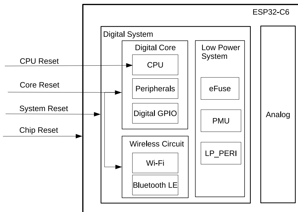
Figure 8.1-1. Reset Types
