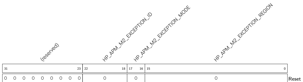
Register 16.16. HP_APM_M2_EXCEPTION_INFO0_REG (0x00F0)
