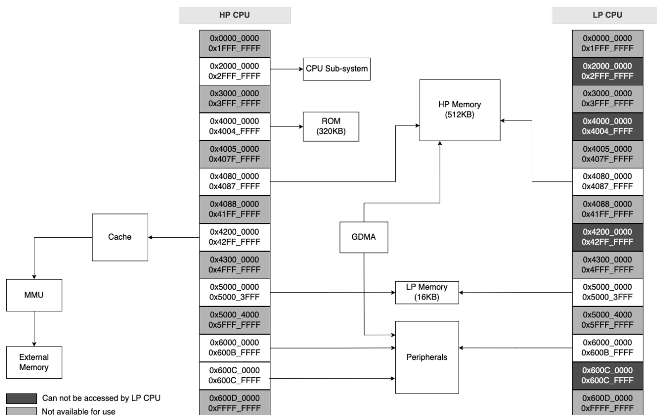
Figure 5.2-1. System Structure and Address Mapping
