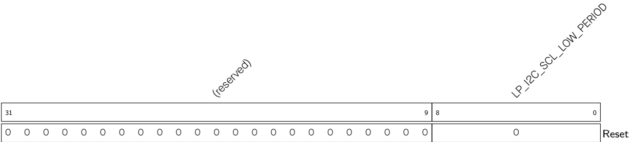
Register 29.36. LP_I2C_SCL_LOW_PERIOD_REG (0x0000)
