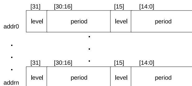
Figure 37.3-2. Format of Pulse Code in RAM
