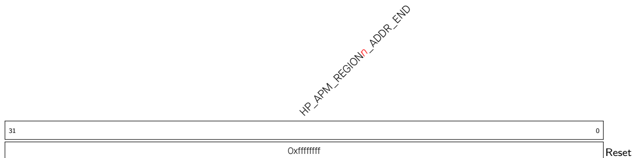
Register 16.3. HP_APM_REGION n _ADDR_END_REG ( n : 0-15) (0x0008+0xC* n )
