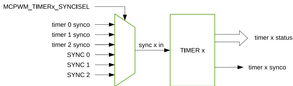
Figure 36.3-2. Timer Module
