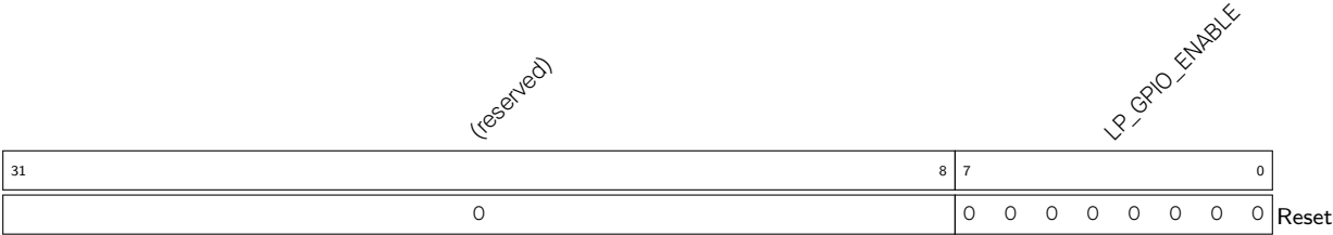
Register 7.38. LP_IO_ENABLE_REG (0x000C)
