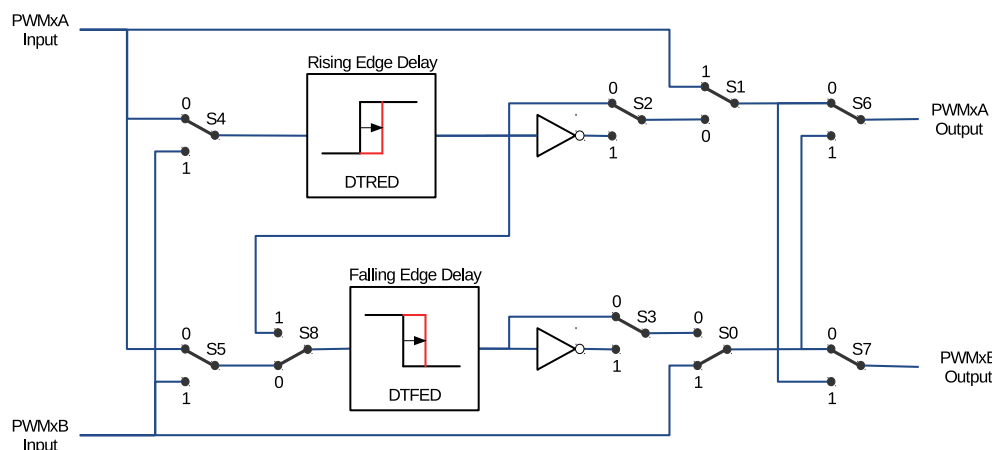
Figure 36.3-23. Options for Setting up the Dead Time Generator Module
