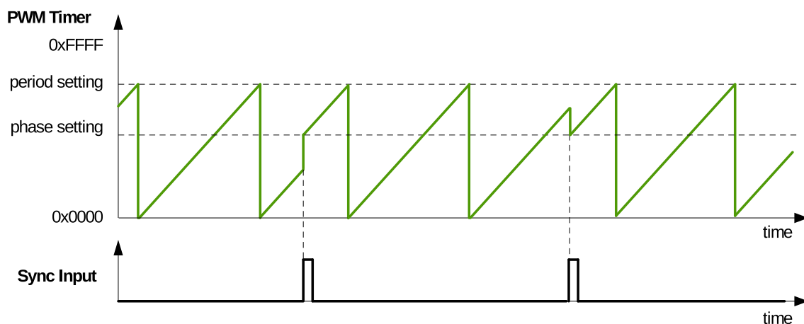
Figure 36.3-7. Count-Up Mode Waveform
