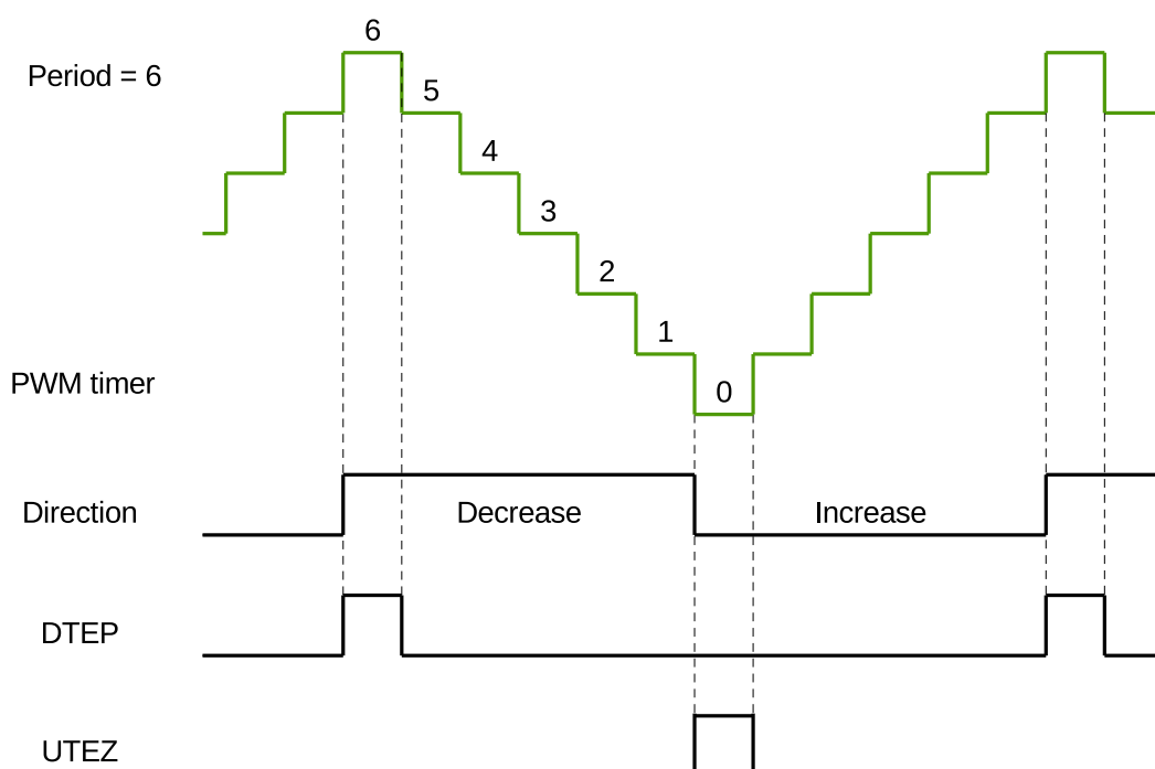
Figure 36.3-13. DTEP and UTEZ Generation in Count-Up-Down Mode
