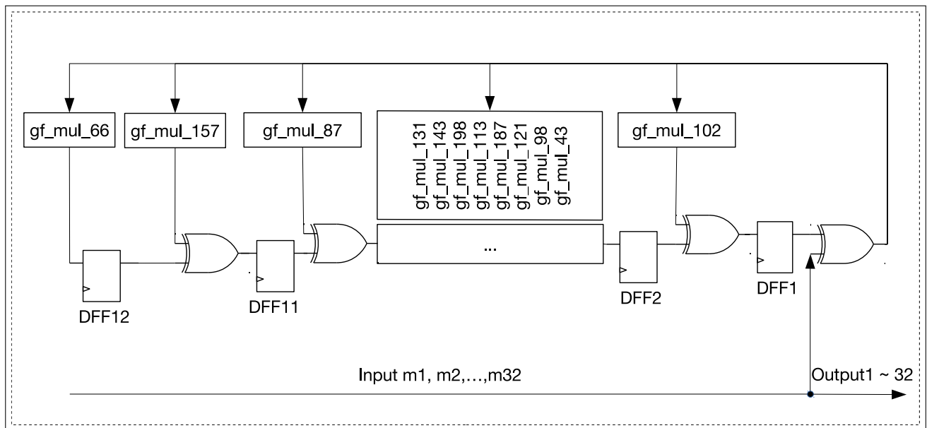
Figure 6.3-2. Shift Register Circuit (first 32 output)
