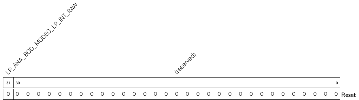
Register 12.87. LP_ANA_LP_INT_RAW_REG (0x0020)
