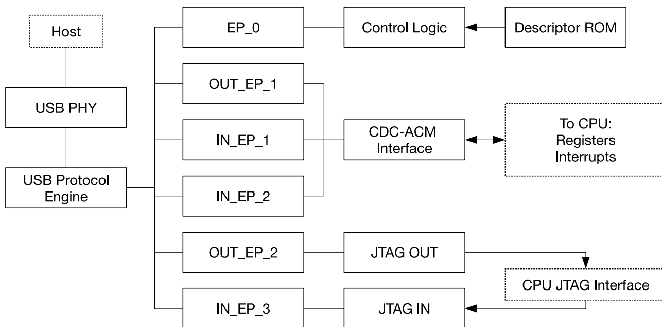
Figure 32.2-2. USB Serial/JTAG Block Diagram
