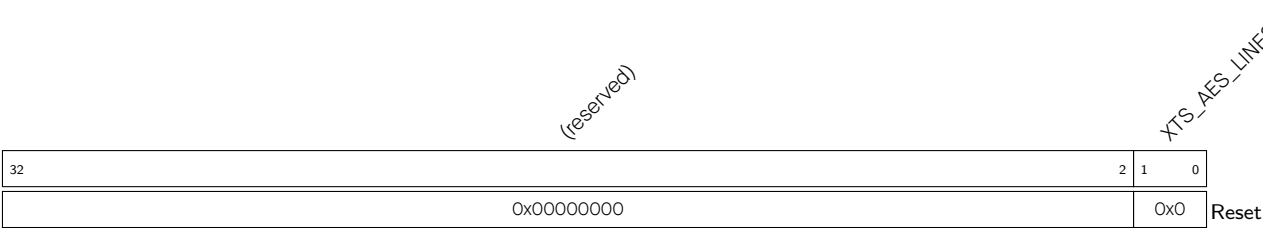
Register 25.2. XTS_AES_LINESIZE_REG (0x0340)
