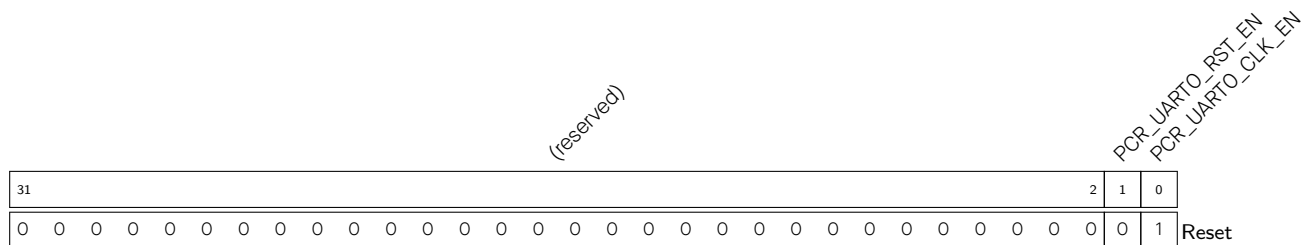
Register 8.1. PCR_UARTO_CONF_REG (0x0000)
