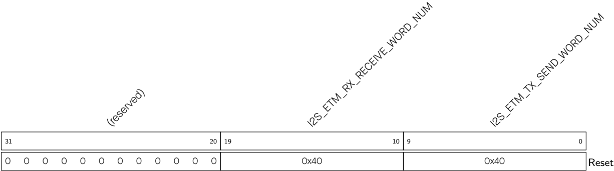
Register 30.19. I2S_ETM_CONF_REG (0x0070)
