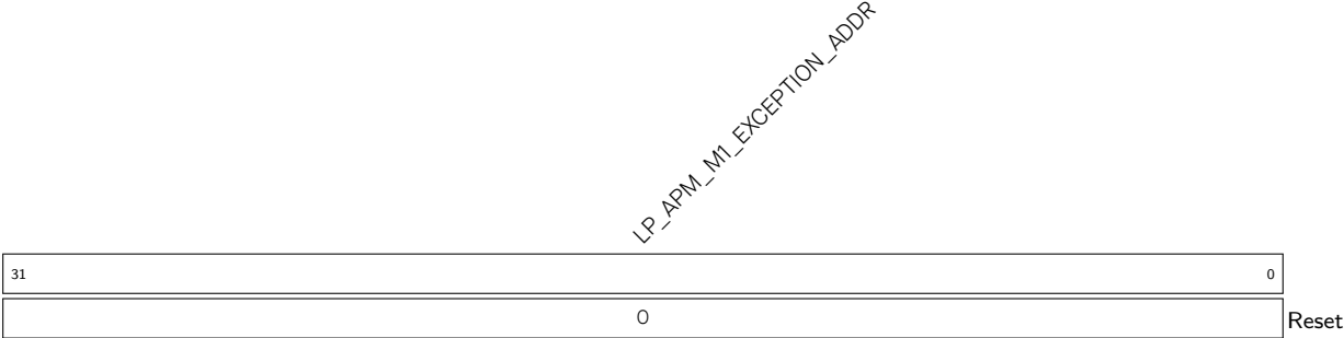
Register 16.37. LP_APM_M1_EXCEPTION_INFO1_REG (0x00E4)
