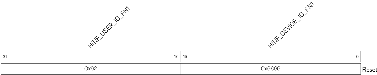
Register 34.1. HINF_CFG_DATA0_REG (0x0000)
