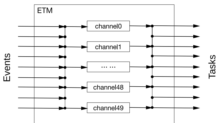
Figure 11.3-1. Event Task Matrix Architecture
