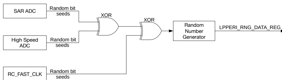
Figure 26.3-1. Noise Source
