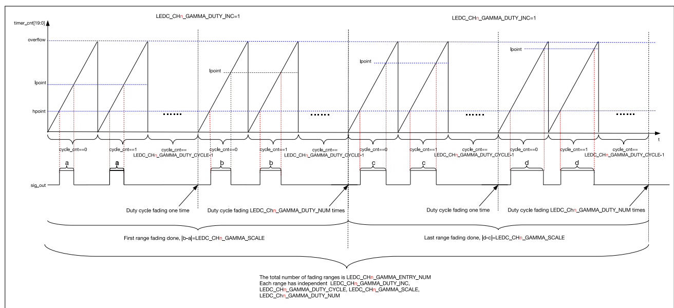
Figure 35.3-6. Output Signal of Gamma Curve Fading
