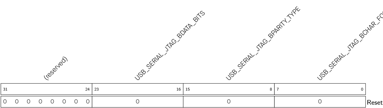
Register 32.26. USB_SERIAL_JTAG_SET_LINE_CODE_W1_REG (0x0054)
