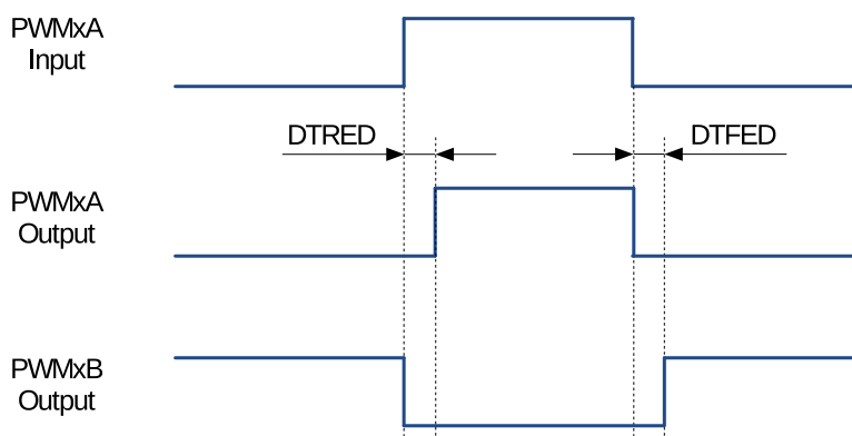
Figure 36.3-24. Active High Complementary (AHC) Dead Time Waveforms
