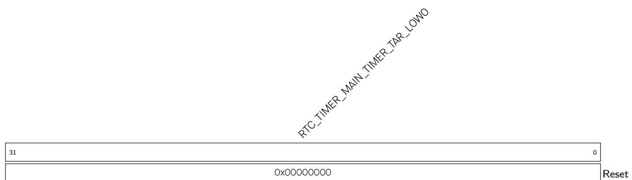
Register 12.63. RTC_TIMER_TARO_LOW_REG (0x0000)
