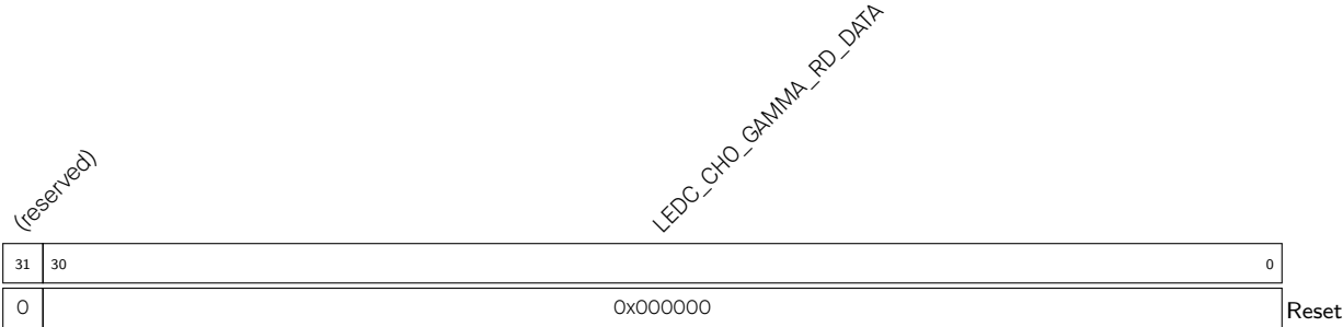
Register 35.21. LEDC_CHn_GAMMA_RD_DATA_REG (n: 0-5) (0x010C+0x10*n)
