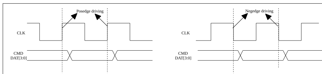
Figure 34.5-9. Output Timing Diagram
