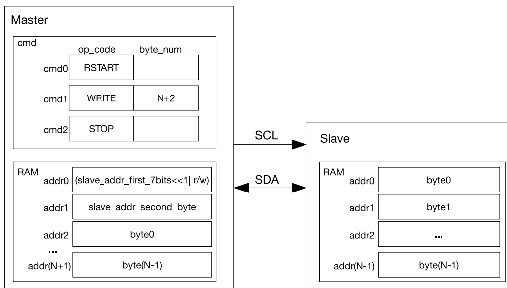
Figure 29.6-2. I2C master Writing to a Slave with a 10-bit Address
