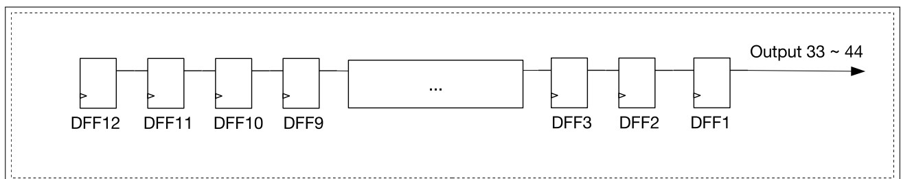
Figure 6.3-3. Shift Register Circuit (last 12 output)
