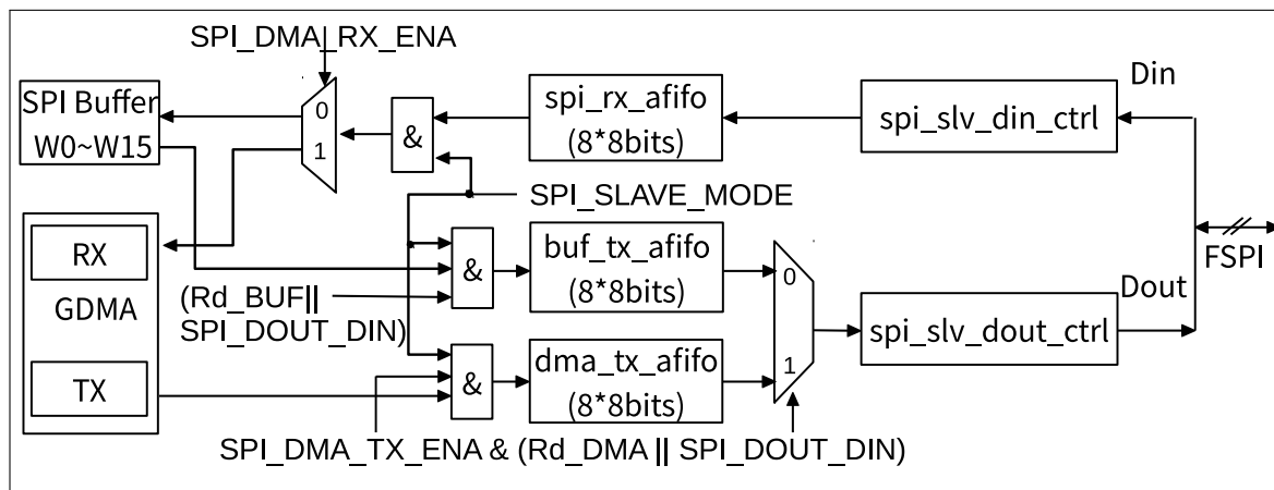
Figure 28.5-4. Data Flow Control in GP-SPI2 as Slave
