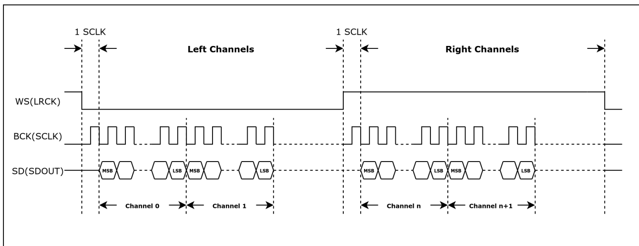
Figure 30.5-1. TDM Philips Standard Timing Diagram
