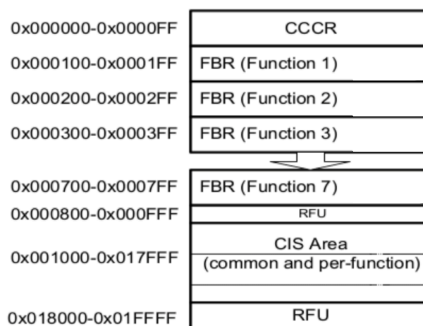
Figure 34.5-3. Function 0 Address Space
