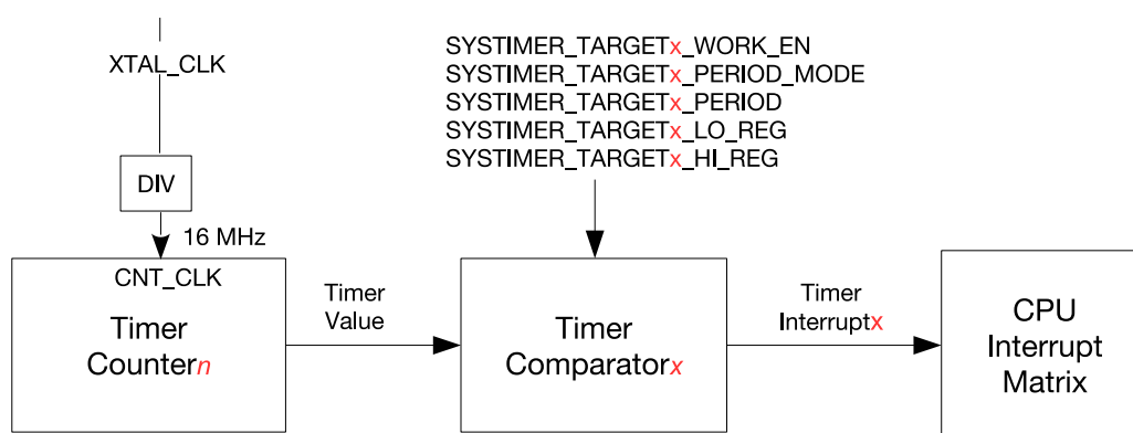
Figure 13.4-1. System Timer Alarm Generation
