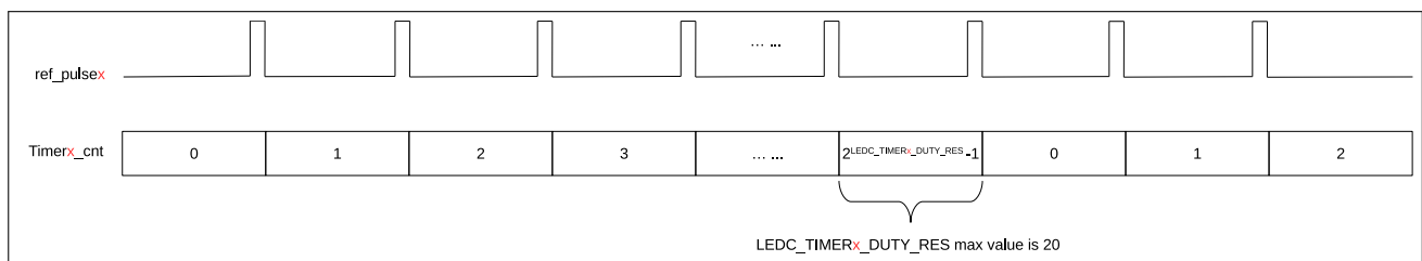
Figure 35.3-3. Relationship Between Counter And Resolution
