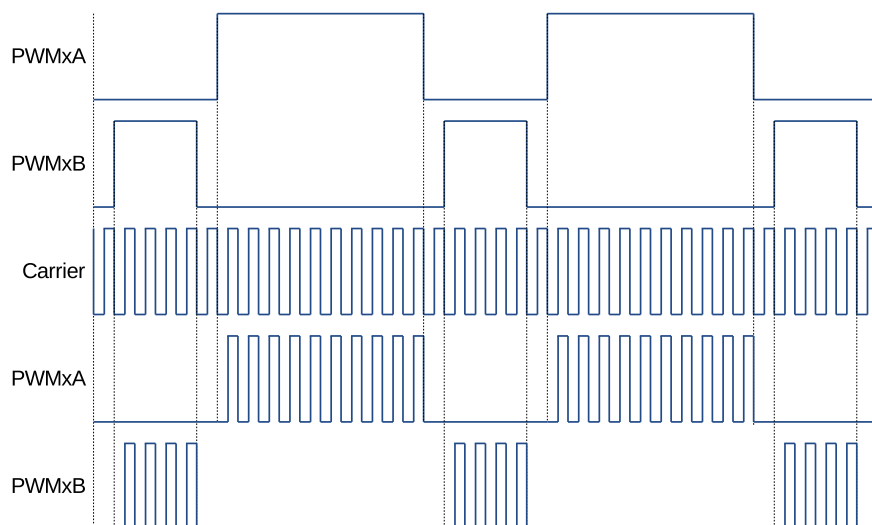
Figure 36.3-28. Example of Waveforms Showing PWM Carrier Action
