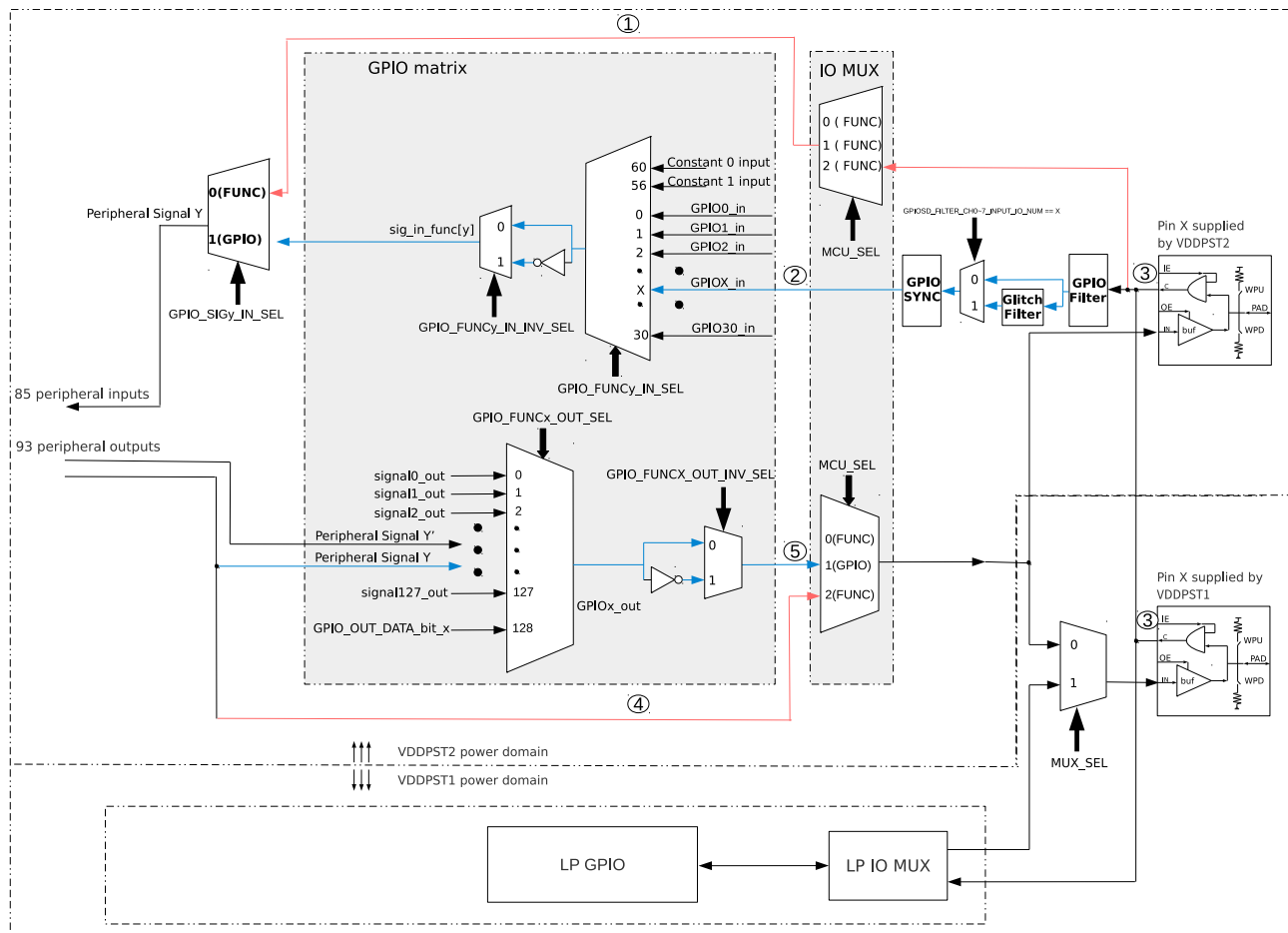
Figure 7.3-1. Architecture of IO MUX, LP IO MUX, and GPIO Matrix
