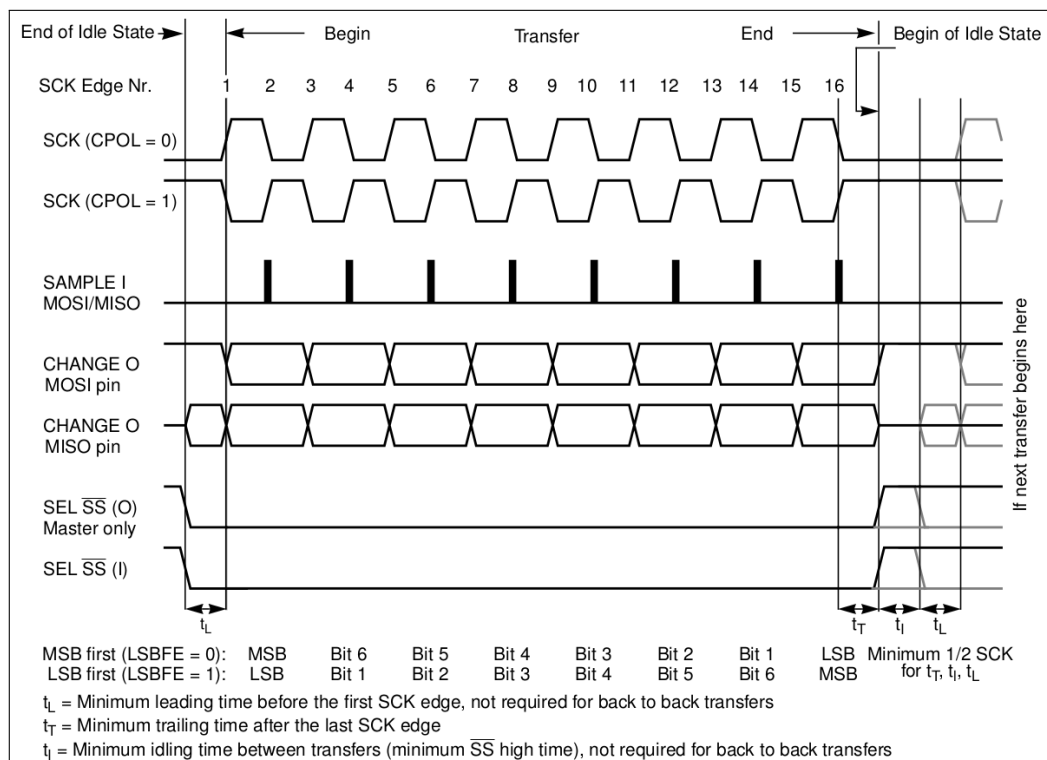
Figure 28.7-2. SPI Clock Mode 1 or 3
