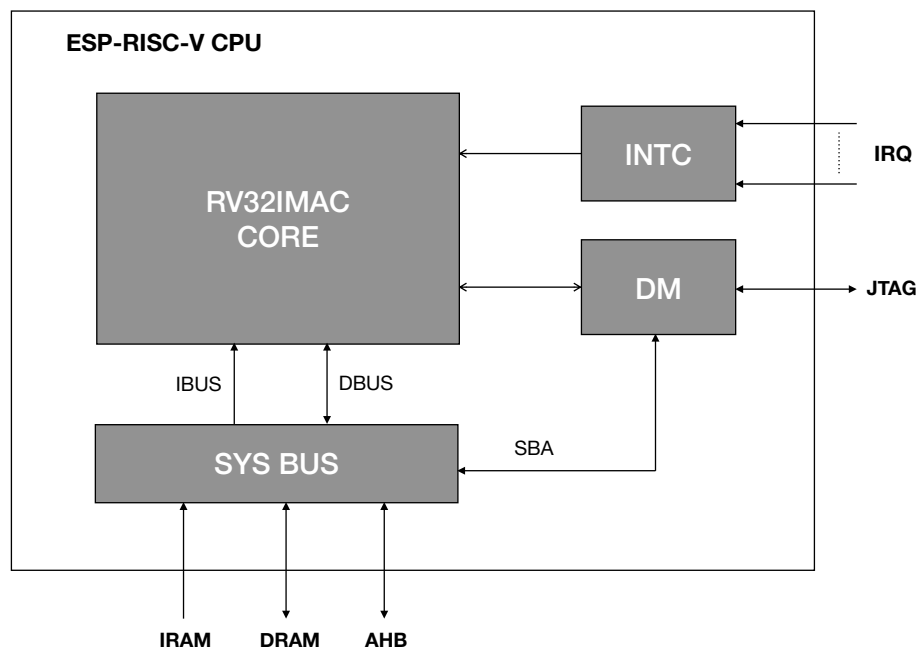
Figure 1.1-1. CPU Block Diagram
