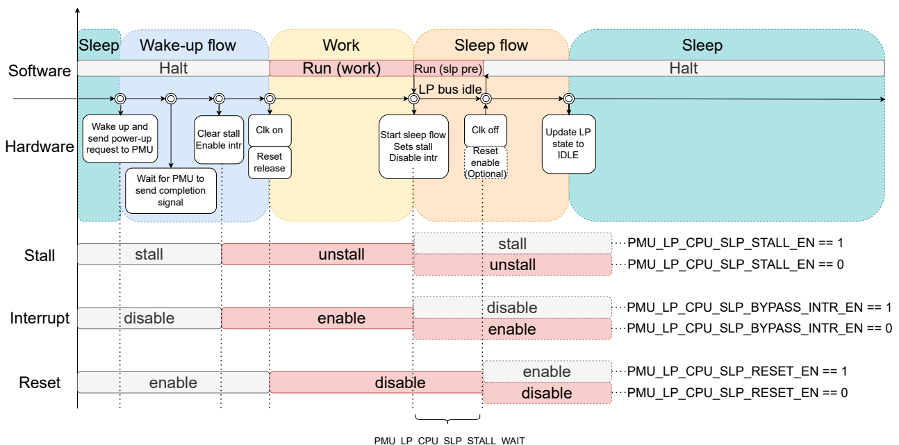
Figure 3.9-1. Wake-Up and Sleep Flow of LP CPU
