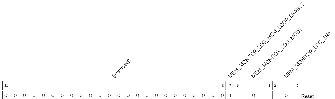
Register 18.1. MEM_MONITOR_LOG_SETTING_REG (0x0000)
