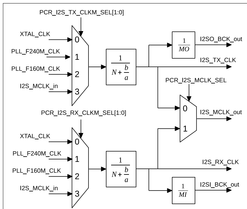
Figure 30.6-1. I2S Clock Generator
