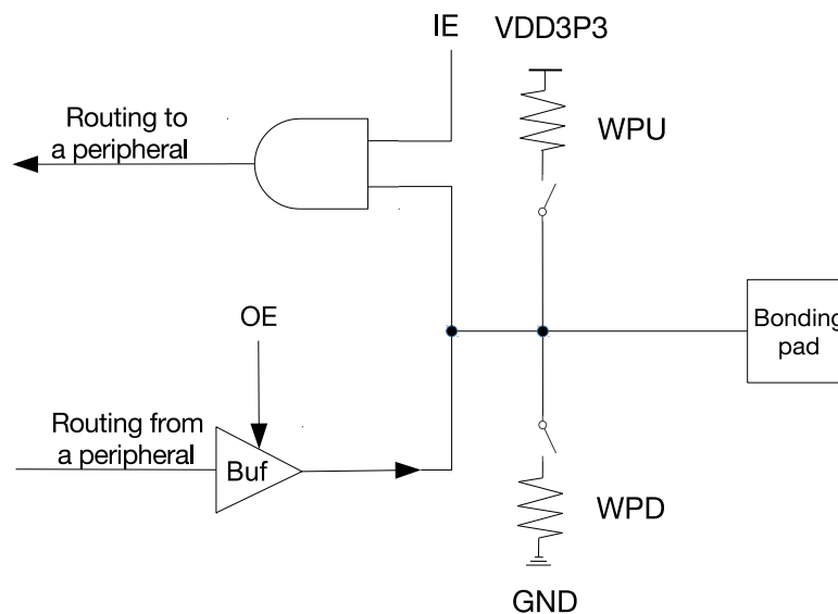
Figure 7.3-2. Internal Structure of a Pad
