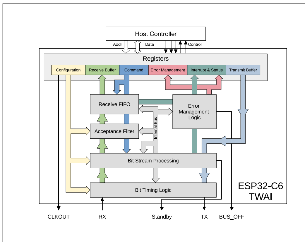
Figure 33.3-1. TWAI Overview Diagram
