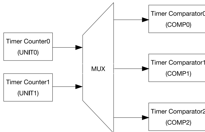
Figure 13.1-1. System Timer Structure
