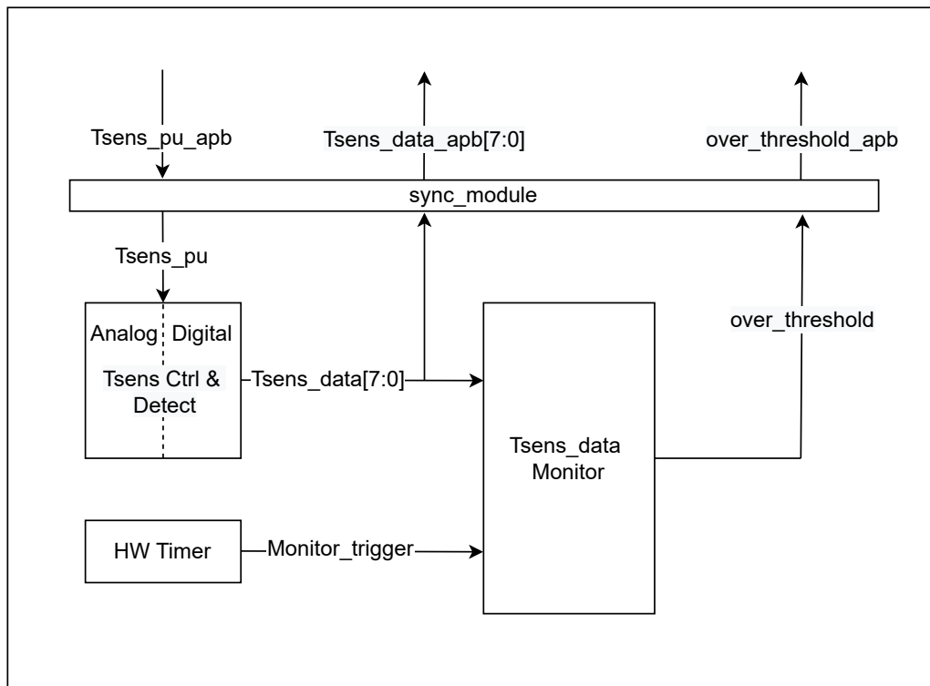
Figure 39.3-1. Temperature Sensor Structure
