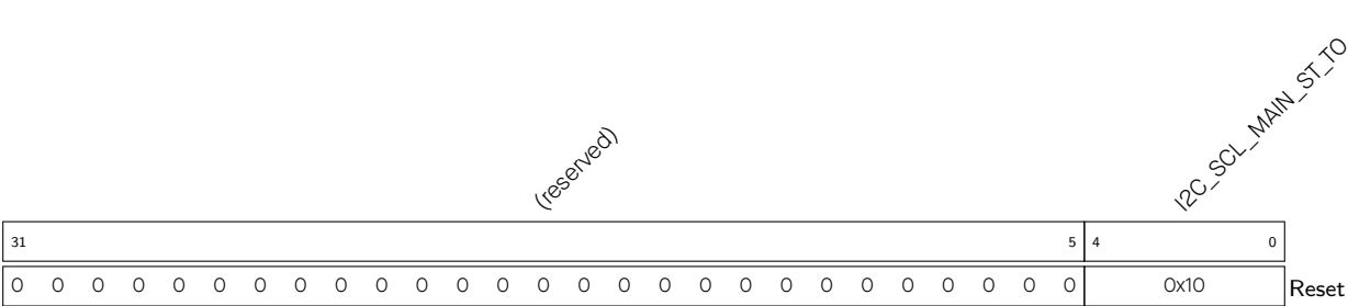
Register 29.10. I2C_SCL_MAIN_ST_TIME_OUT_REG (0x007C)
