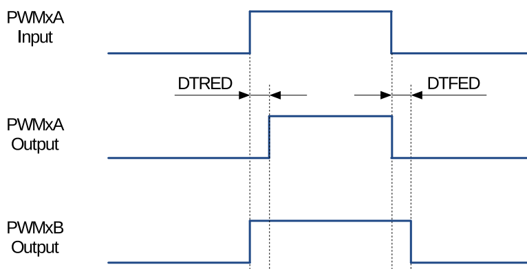
Figure 36.3-26. Active High (AH) Dead Time Waveforms
