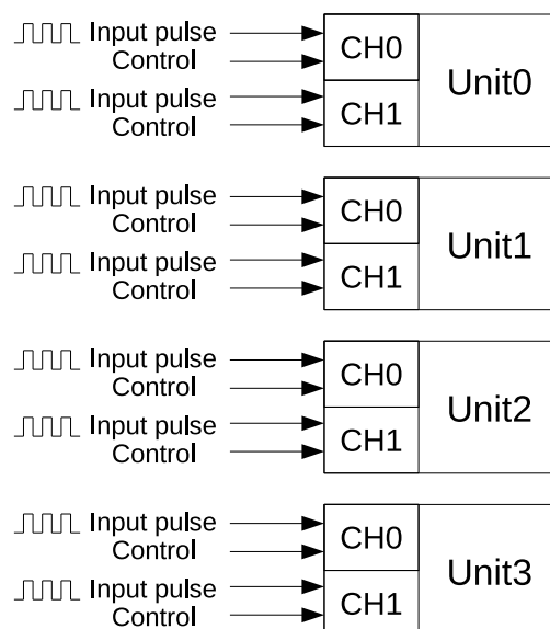
Figure 31.0-1. PCNT Block Diagram
