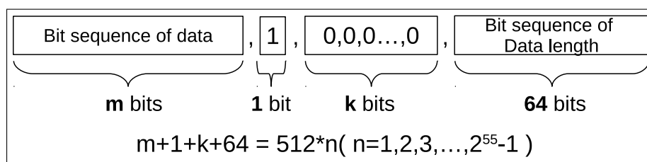
Figure 21.3-1. HMAC SHA-256 Padding Diagram
