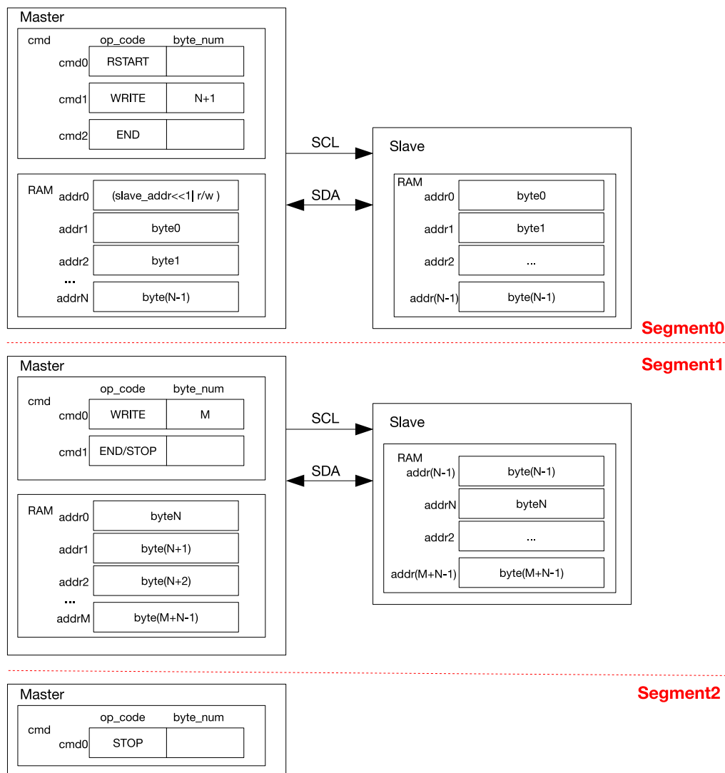
Figure 29.6-4. I2C master Writing to I2C slave with a 7-bit Address in Multiple Sequences
