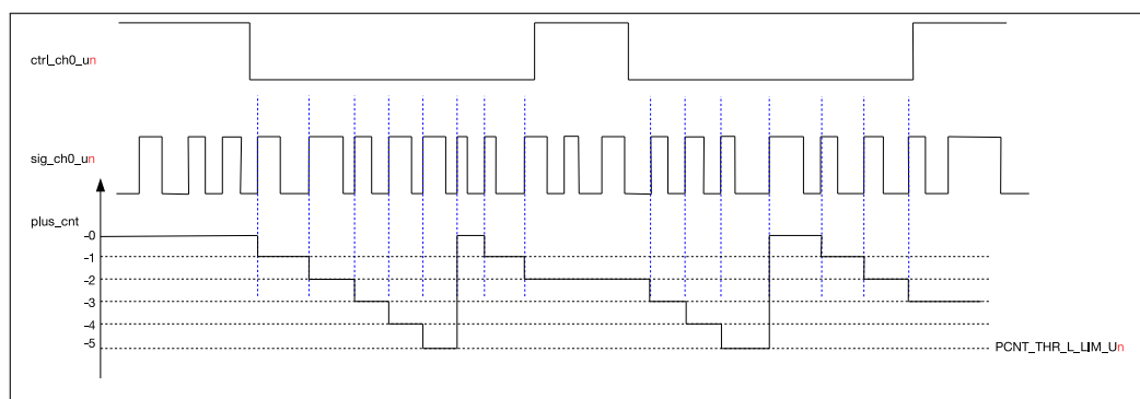
Figure 31.3-2. Channel 0 Down Counting Diagram
