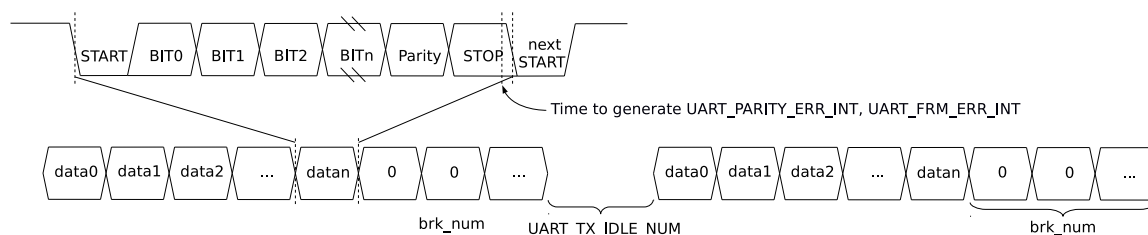
Figure 27.4-3. Structure of UART Data Frame
