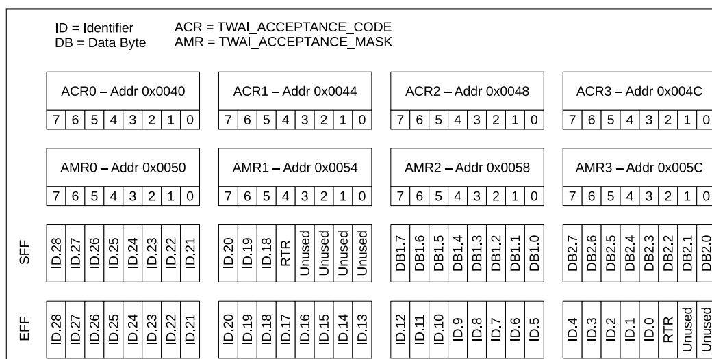
Figure 33.4-2. Single Filter Mode
