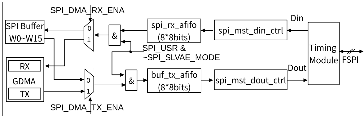
Figure 28.5-3. Data Flow Control in GP-SPI2 as Master
