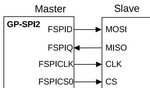
Figure 28.5-6. Full-Duplex Communication Between GP-SPI2 Master and a Slave
