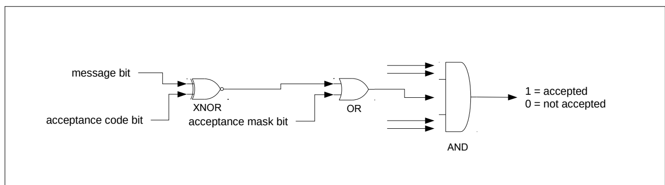
Figure 33.4-1. Acceptance Filter
