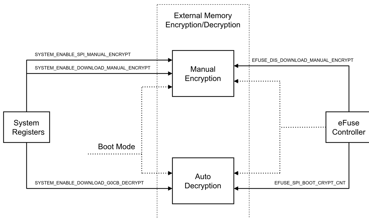
Figure 25.3-1. Architecture of the External Memory Encryption and Decryption
