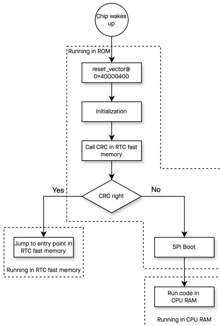
Figure 12.6-1. ESP32-C6 Boot Flow
