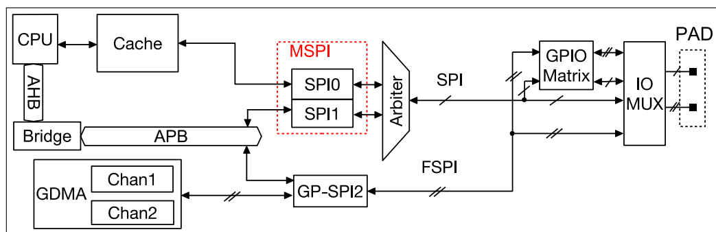
Figure 28.4-1. SPI Module Overview
