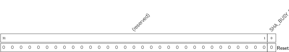
Register 23.3. SHA_BUSY_REG (0x0018)
