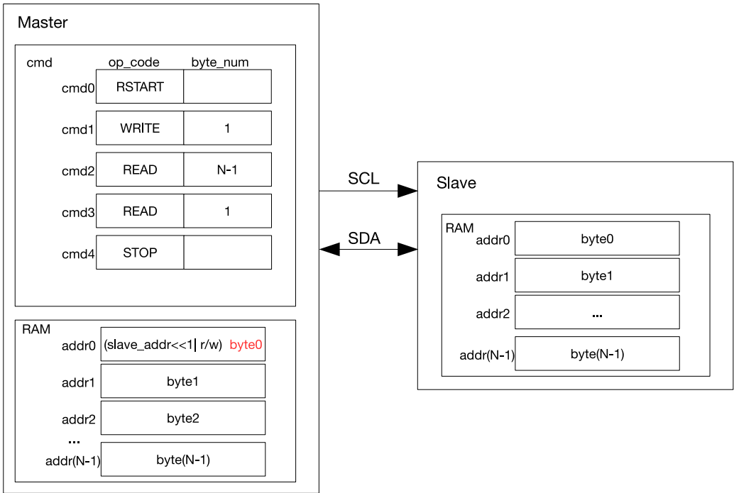
Figure 29.6-5. I2C master Reading I2C slave with a 7-bit Address
