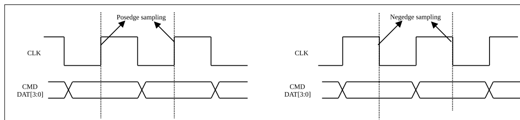
Figure 34.5-8. Sampling Timing Diagram
