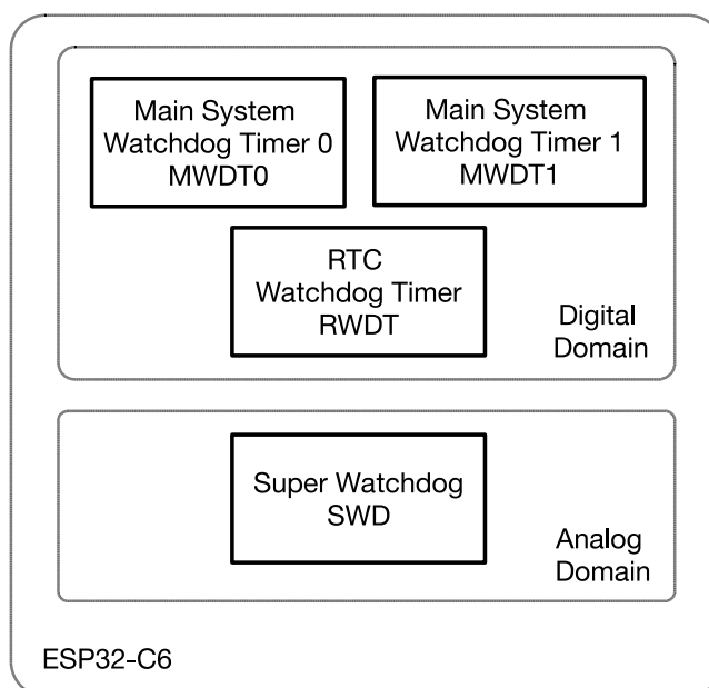
Figure 15.1-1. Watchdog Timers Overview
