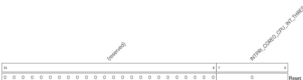
Register 10.68. INTPRI_CORE0_CPU_INT_THRESH_REG (0x008C)
