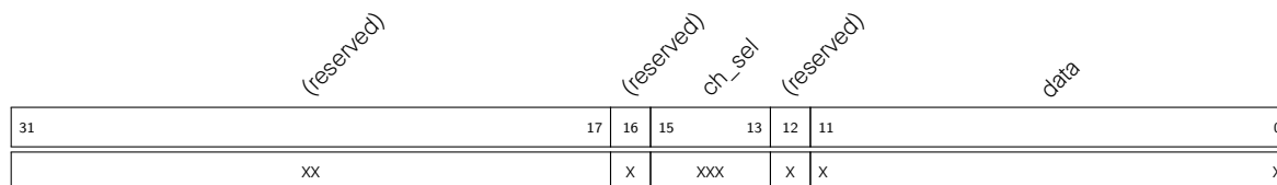
Figure 39.2-8. DMA Data Format
