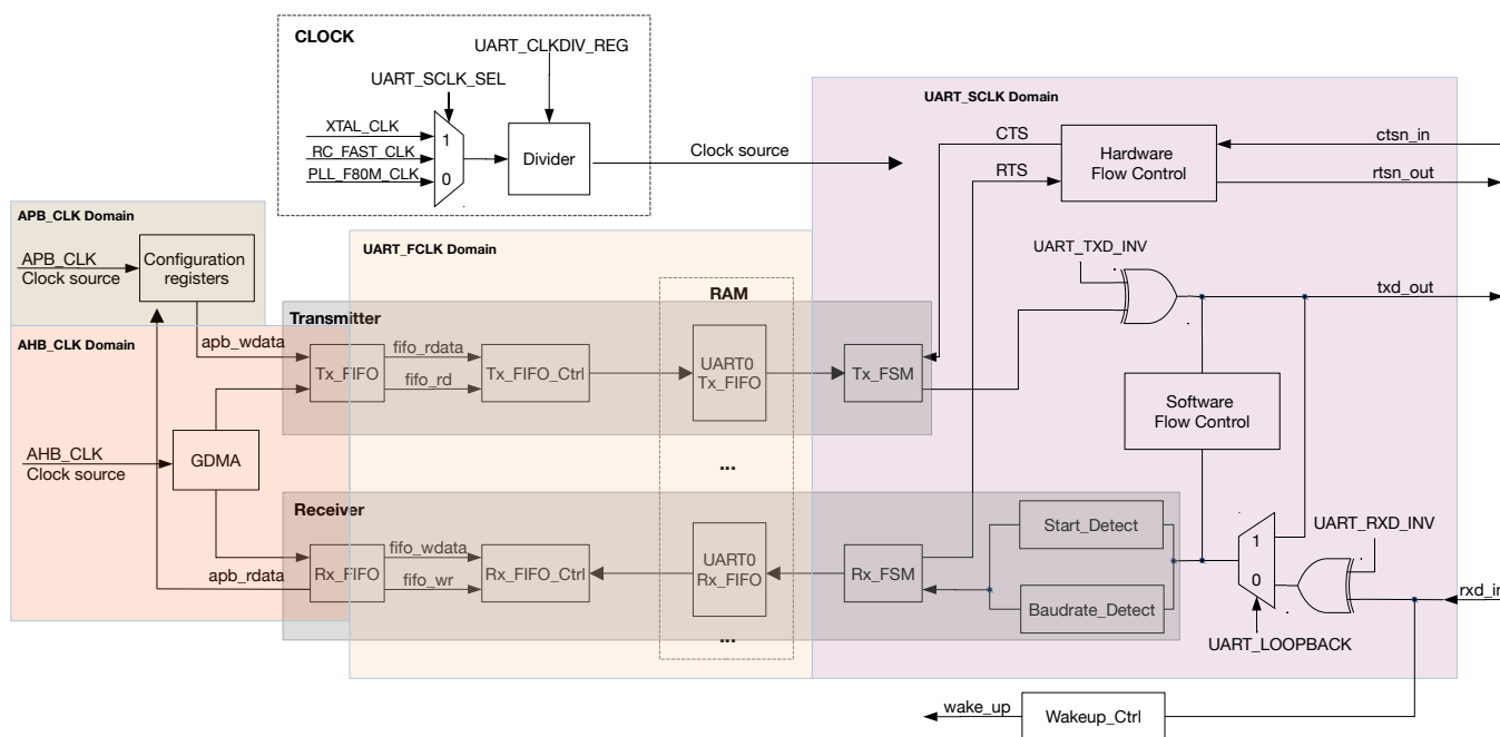
Figure 27.3-1. UART Structure
