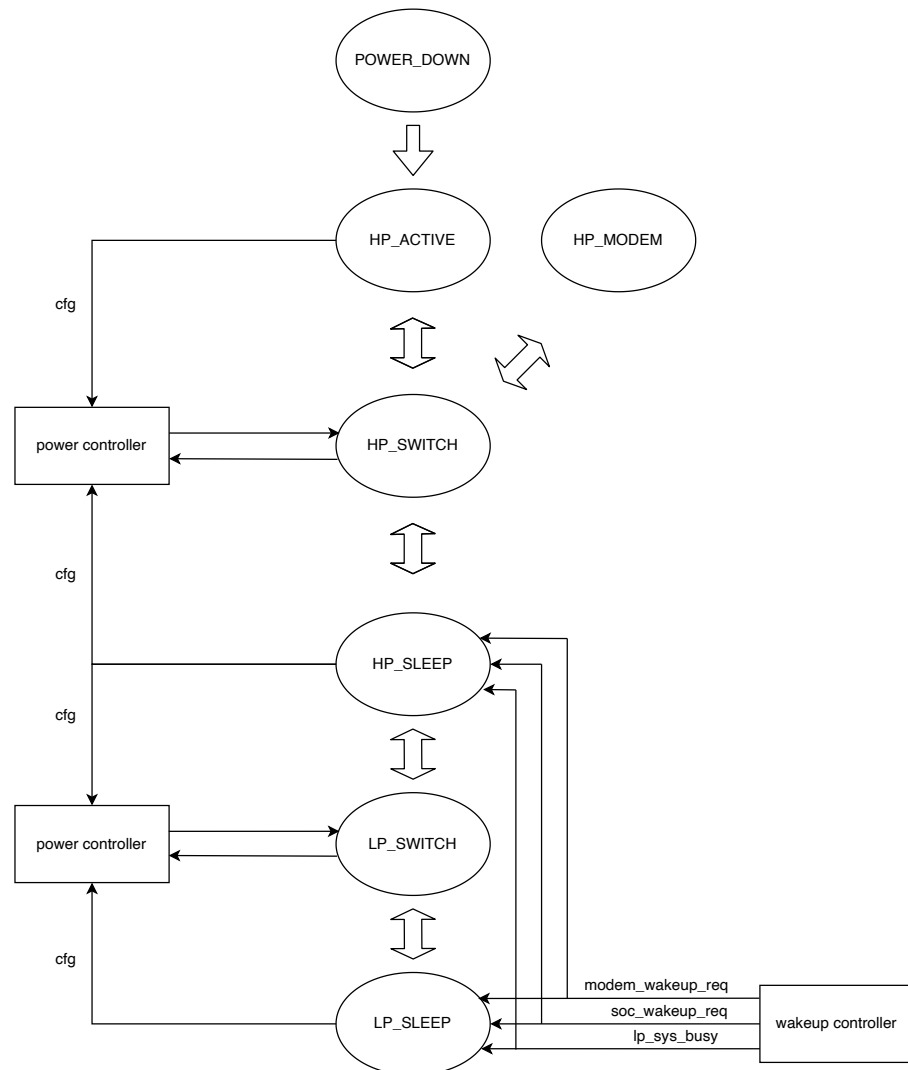
Figure 12.4-2. PMU Workflow
