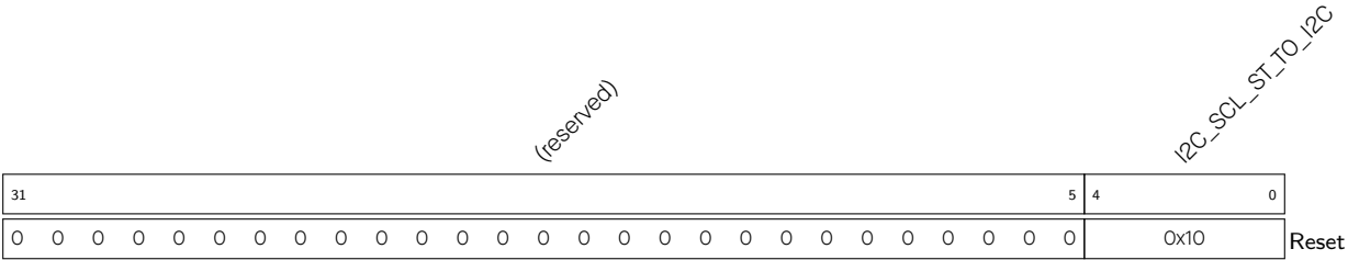
Register 29.9. I2C_SCL_ST_TIME_OUT_REG (0x0078)
