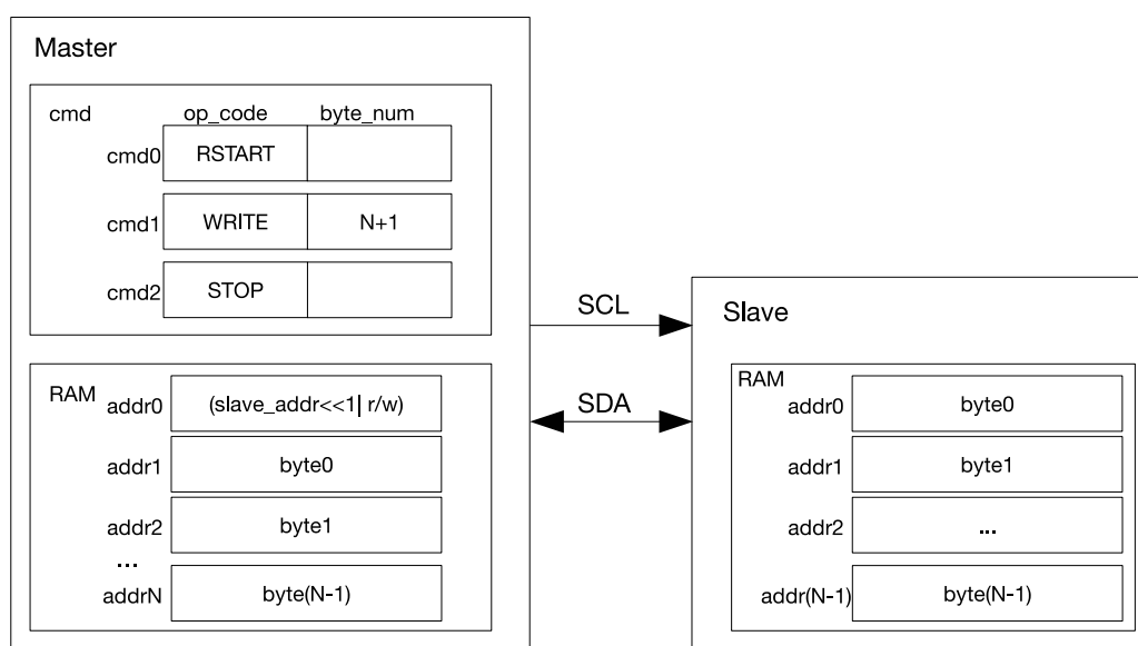
Figure 29.6-1. I2C master Writing to I2C slave with a 7-bit Address
