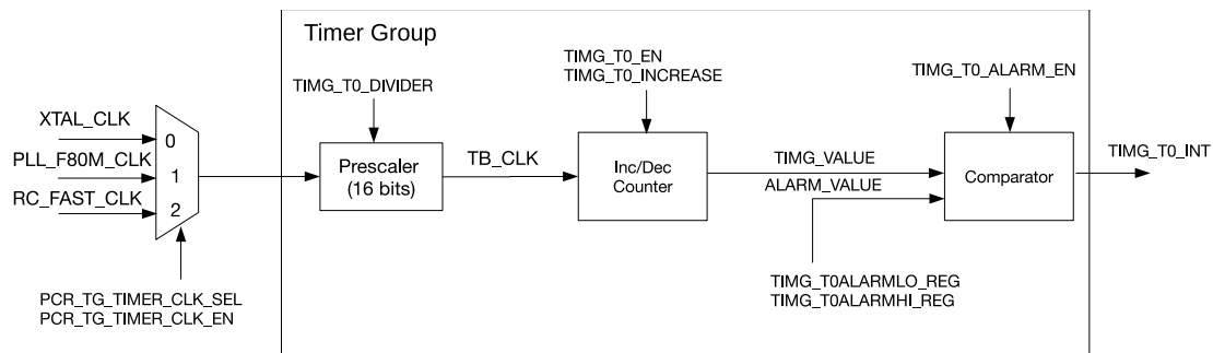
Figure 14.3-1. Timer Group Architecture
