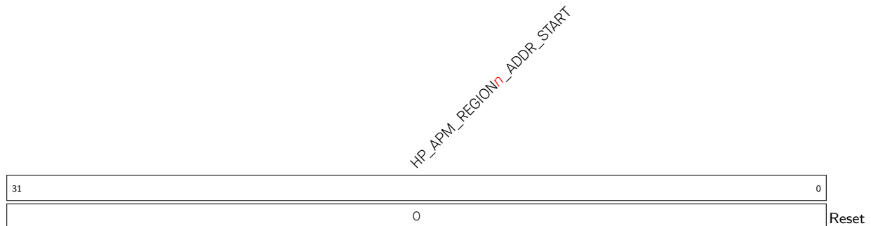
Register 16.2. HP_APM_REGION n _ADDR_START_REG ( n : 0-15) (0x0004+0xC* n )
