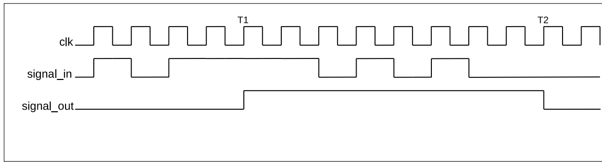
Figure 7.4-3. Glitch Filter Timing Example
