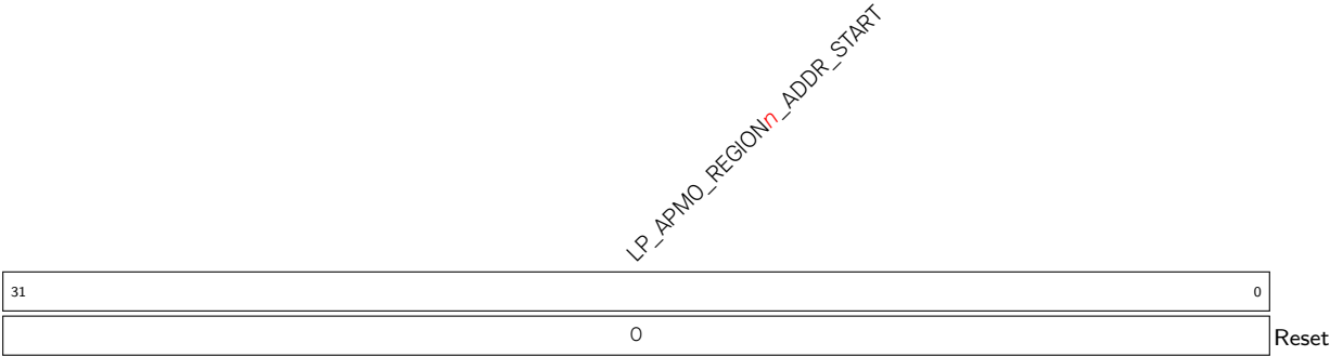
Register 16.42. LP_APM0_REGION n _ADDR_START_REG ( n : 0-3) (0x0004+0xC* n )
