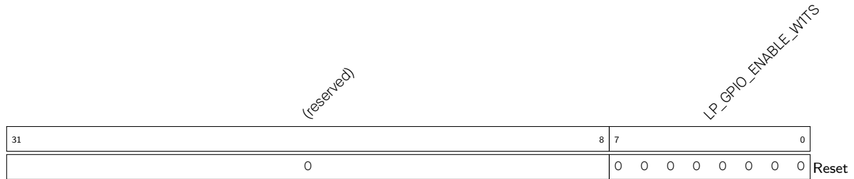
Register 7.39. LP_IO_ENABLE_W1TS_REG (0x0010)
