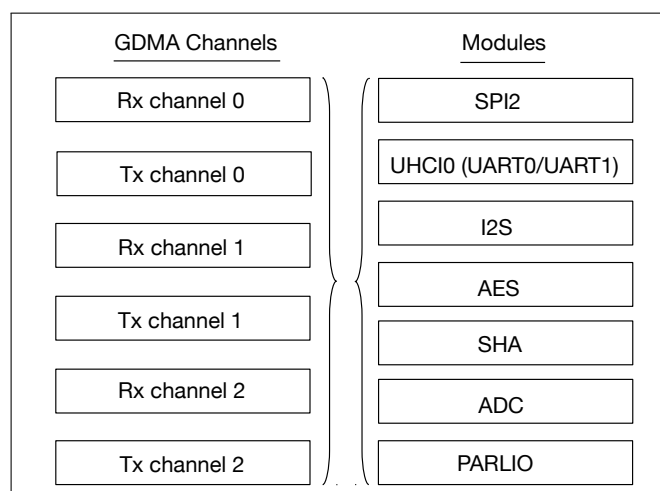
Figure 4.1-1. Modules with GDMA Feature and GDMA Channels
