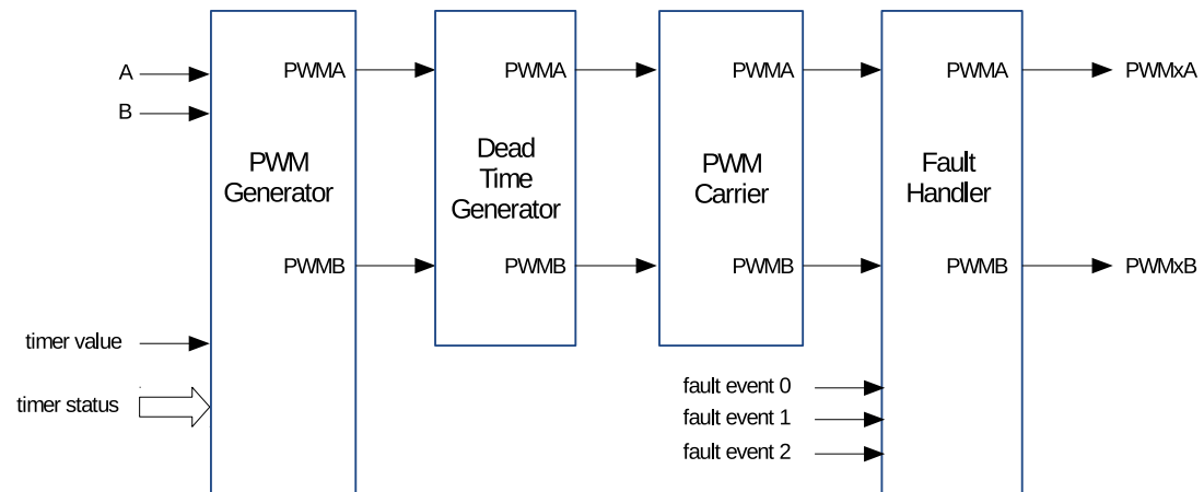
Figure 36.3-14. Block Diagram of A PWM Operator
