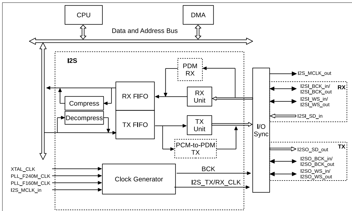
Figure 30.4-1. ESP32-C6 I2S System Diagram
