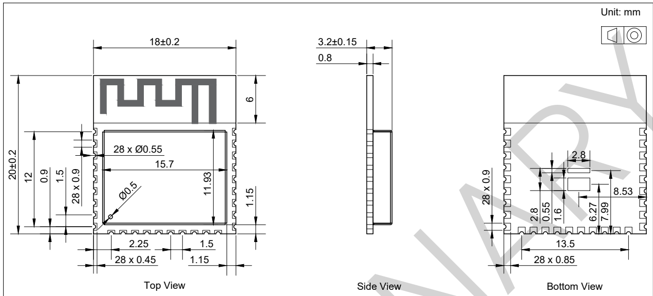
Figure 6: Physical Dimensions
