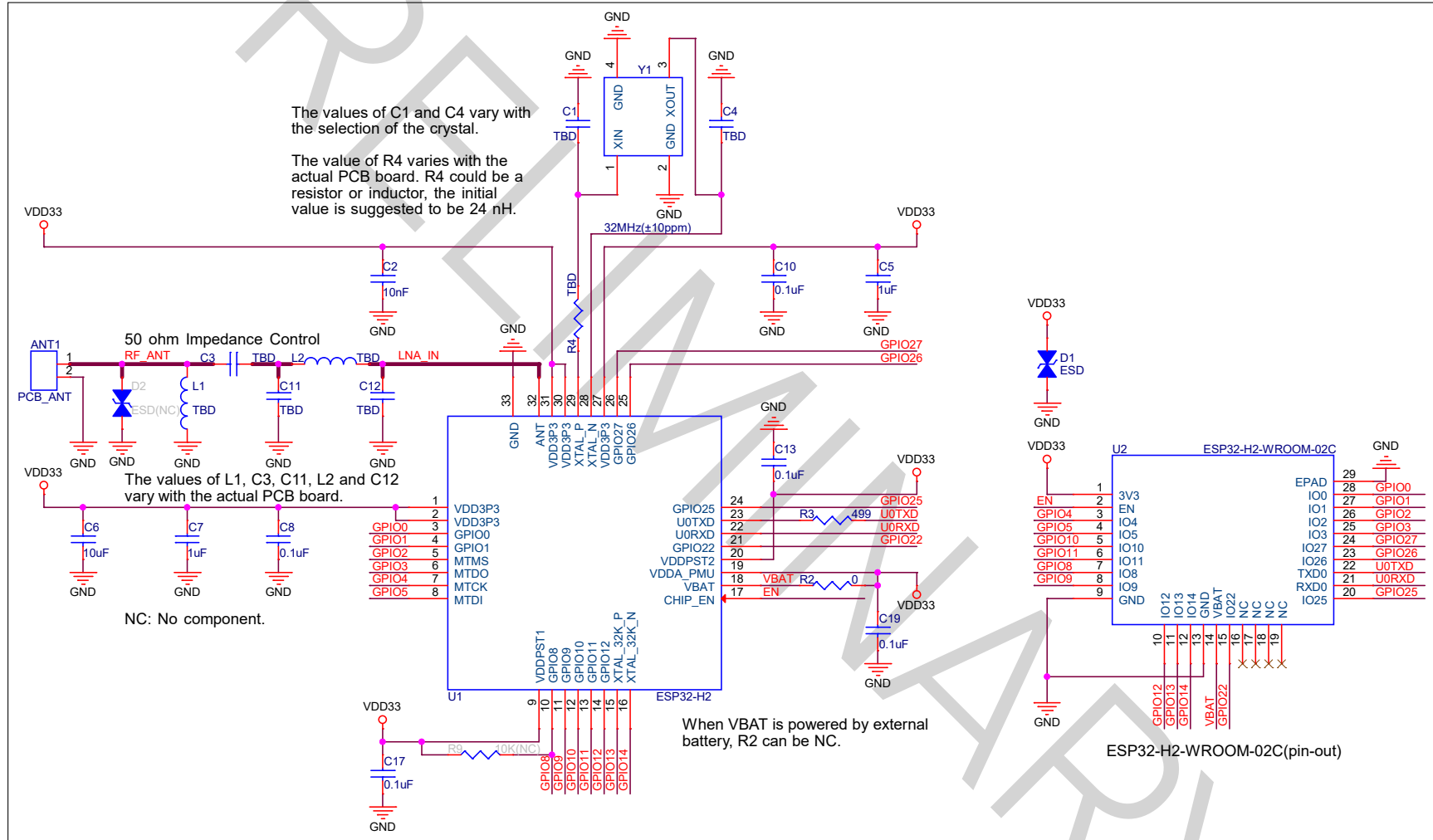
Figure 4: Schematics
