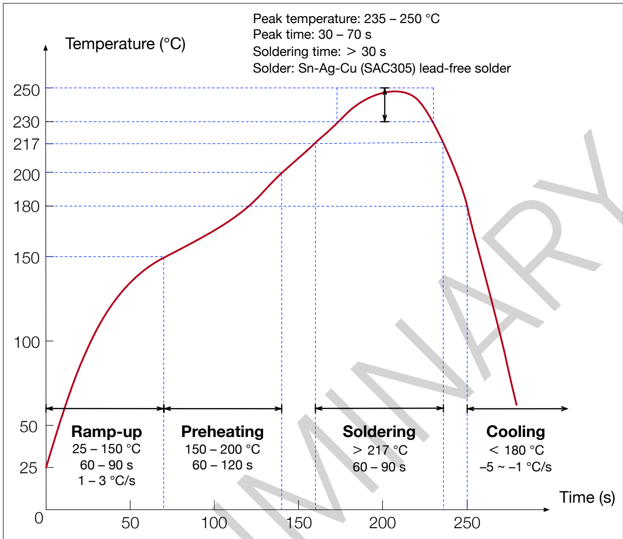
Figure 8: Reflow Profile
