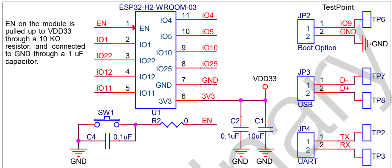
Figure 5: Peripheral Schematics
