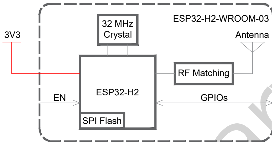
Figure 1: Block Diagram
