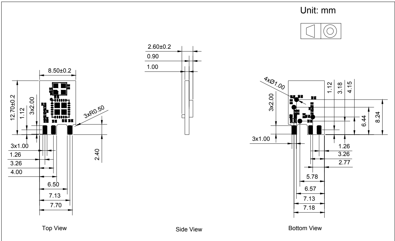
Figure 6: Physical Dimensions
