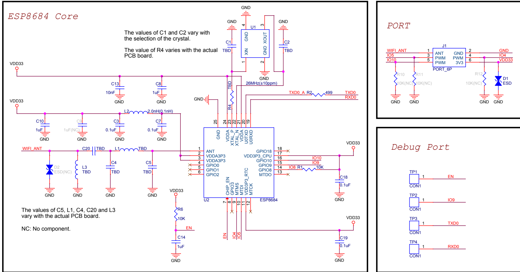
Figure 4: ESP8684-WROOM-07 Schematics
