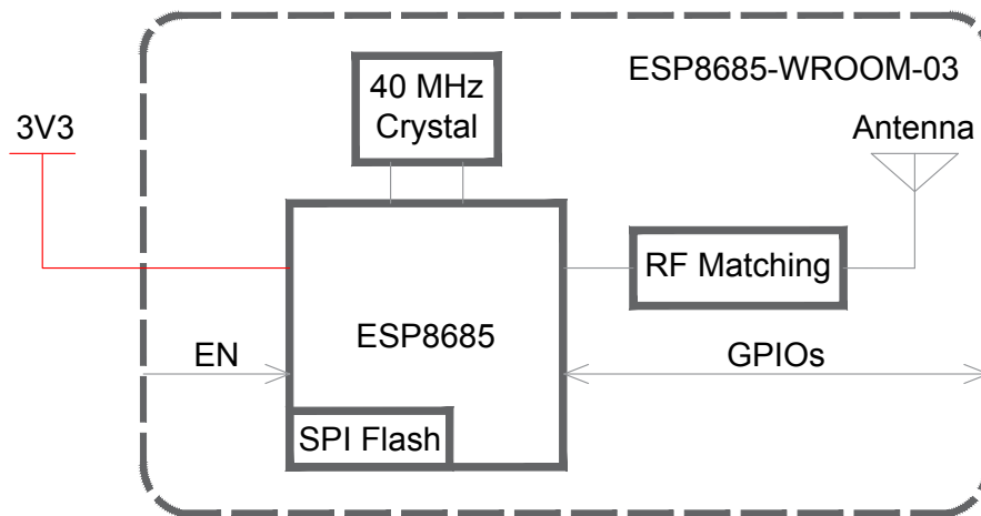
Figure 1: ESP8685-WROOM-03 Block Diagram
