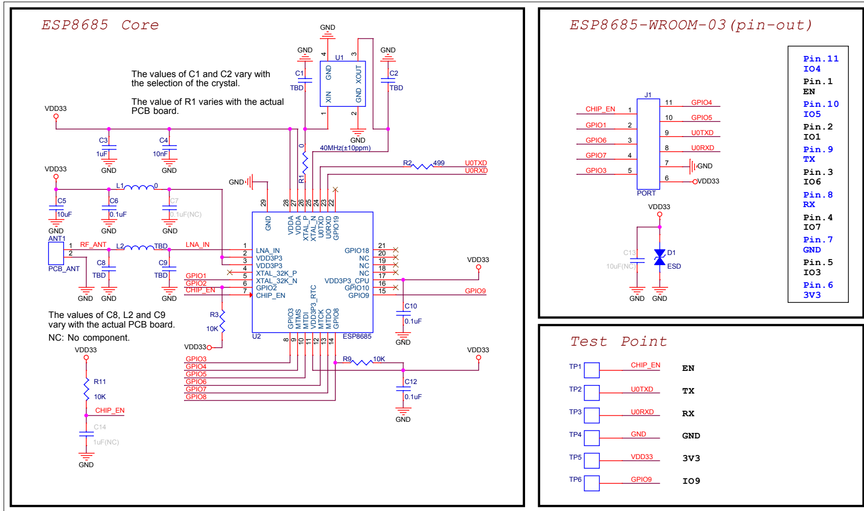
Figure 4: ESP8685-WROOM-03 Schematics
