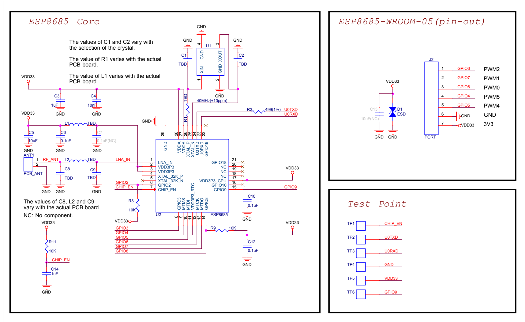
Figure 4: ESP8685-WROOM-05 Schematics
