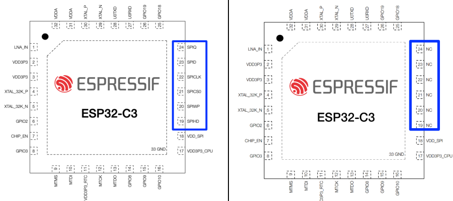
Figure 2-2. ESP32-C3FH4X and ESP32-C3FH4AZ Pin Layout (Top View)
